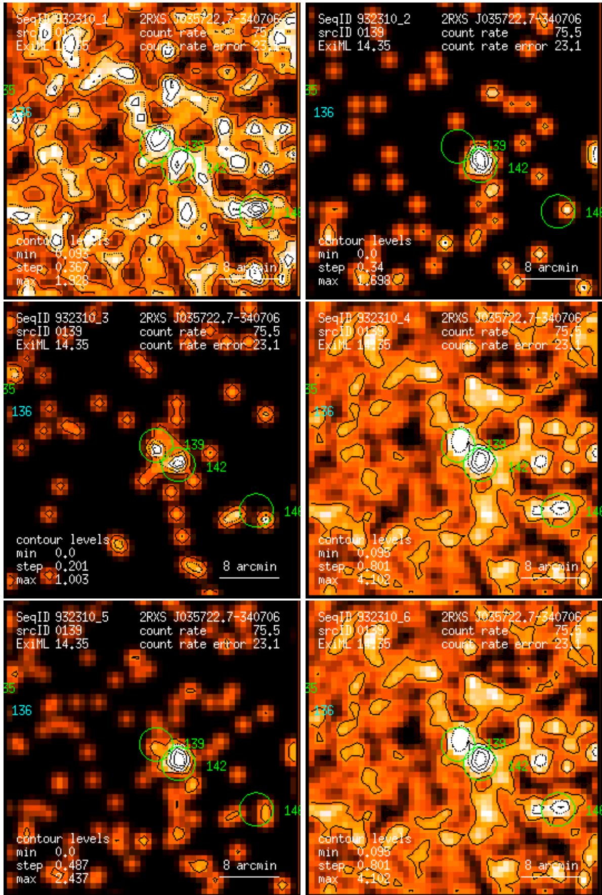
Figure 139: RASS 932310: detection 0139: band rate images, Gaussian filter: (1) PSPC channels 11 – 41, (2) 52 – 90, (3) 91 – 201, (4) 11 – 235, (5) 52 – 201, (6) 11 – 201. Broad band rates in counts/ks. Band rate contour levels in counts/ks/arcmin 2 .
