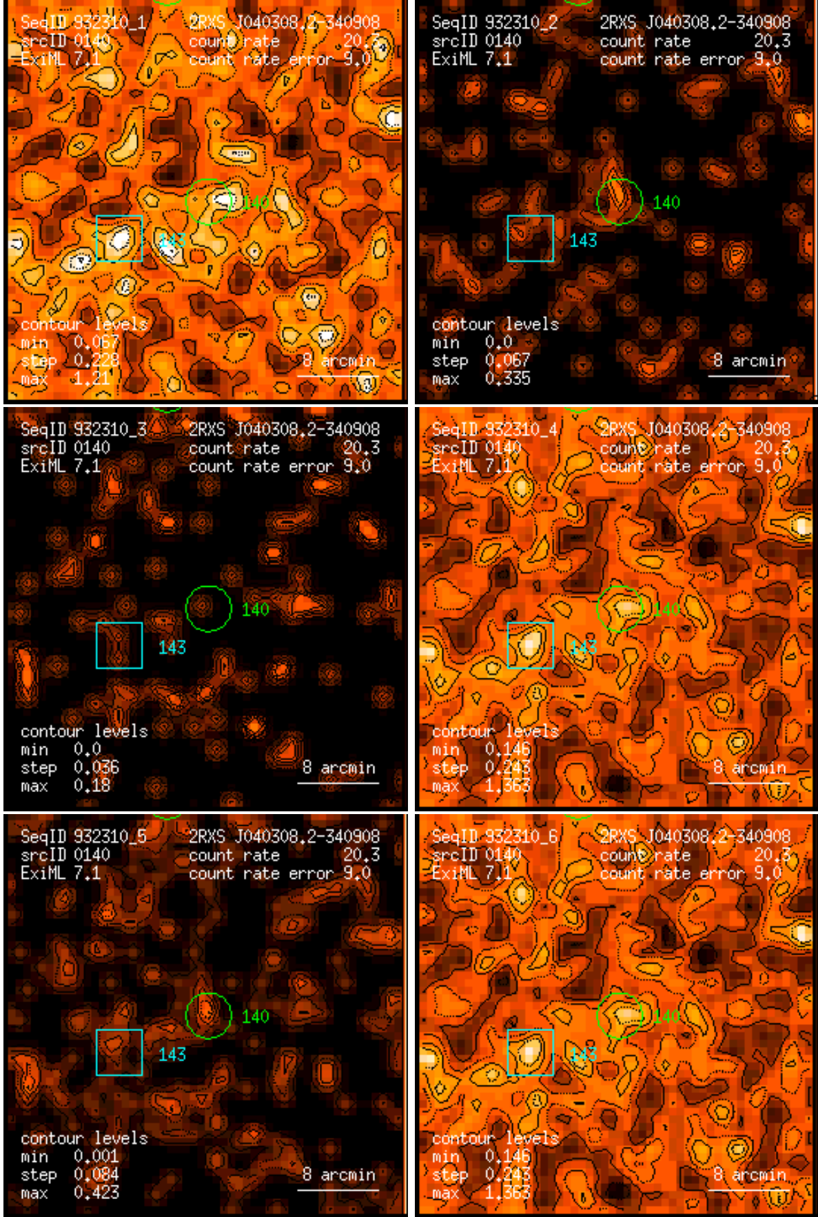
Figure 140: RASS 932310: detection 0140: band rate images, Gaussian filter: (1) PSPC channels 11 – 41, (2) 52 – 90, (3) 91 – 201, (4) 11 – 235, (5) 52 – 201, (6) 11 – 201. Broad band rates in counts/ks. Band rate contour levels in counts/ks/arcmin 2 .
