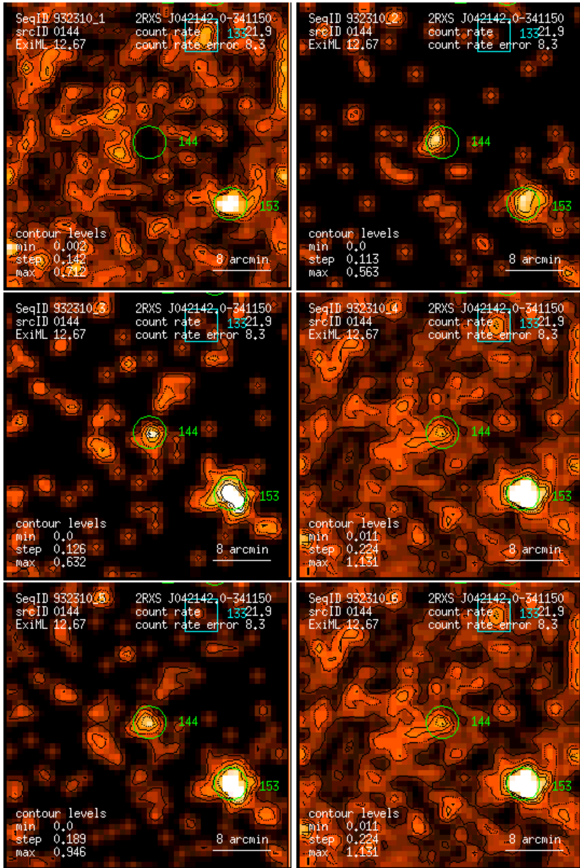
Figure 144: RASS 932310: detection 0144: band rate images, Gaussian filter: (1) PSPC channels 11 – 41, (2) 52 – 90, (3) 91 – 201, (4) 11 – 235, (5) 52 – 201, (6) 11 – 201. Broad band rates in counts/ks. Band rate contour levels in counts/ks/arcmin 2 .
