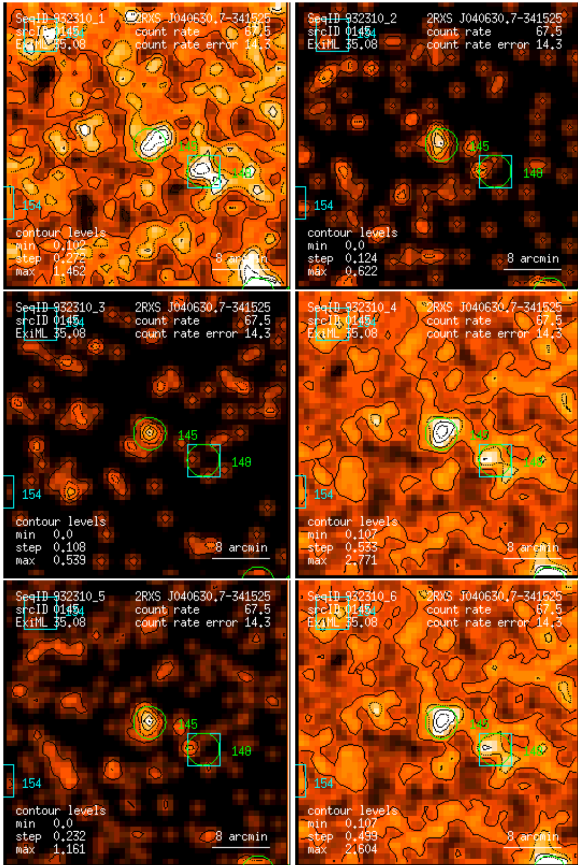
Figure 145: RASS 932310: detection 0145: band rate images, Gaussian filter: (1) PSPC channels 11 – 41, (2) 52 – 90, (3) 91 – 201, (4) 11 – 235, (5) 52 – 201, (6) 11 – 201. Broad band rates in counts/ks. Band rate contour levels in counts/ks/arcmin 2 .
