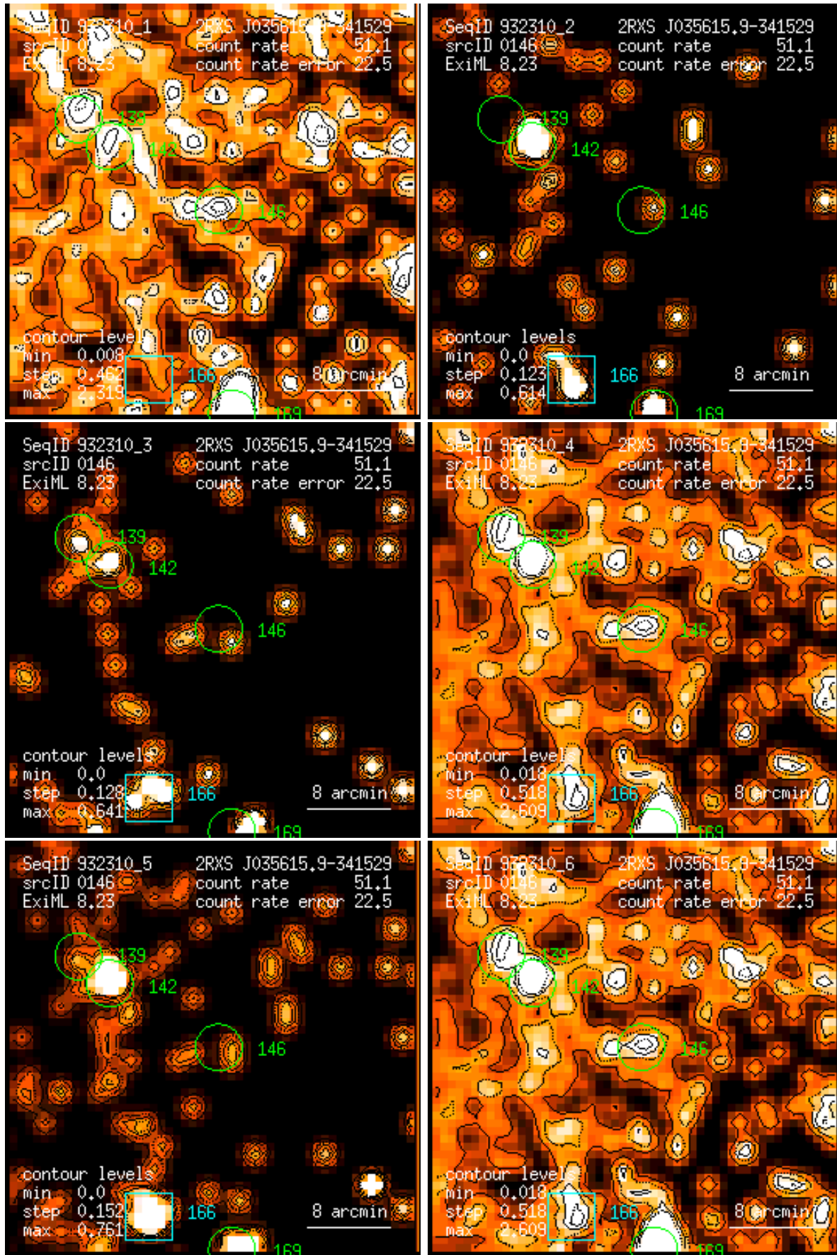
Figure 146: RASS 932310: detection 0146: band rate images, Gaussian filter: (1) PSPC channels 11 – 41, (2) 52 – 90, (3) 91 – 201, (4) 11 – 235, (5) 52 – 201, (6) 11 – 201. Broad band rates in counts/ks. Band rate contour levels in counts/ks/arcmin 2 .
