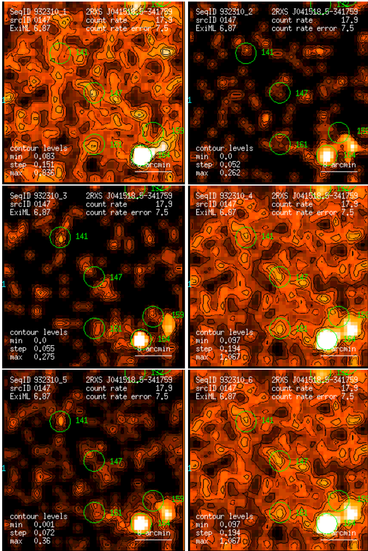
Figure 147: RASS 932310: detection 0147: band rate images, Gaussian filter: (1) PSPC channels 11 – 41, (2) 52 – 90, (3) 91 – 201, (4) 11 – 235, (5) 52 – 201, (6) 11 – 201. Broad band rates in counts/ks. Band rate contour levels in counts/ks/arcmin 2 .
