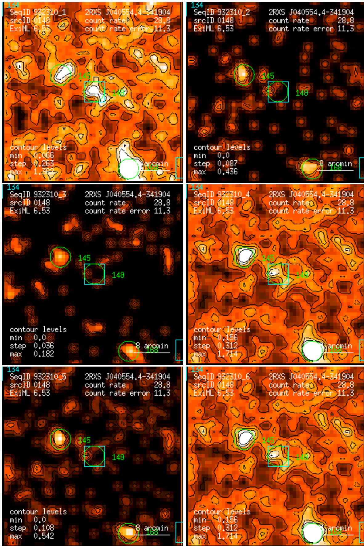
Figure 148: RASS 932310: detection 0148: band rate images, Gaussian filter: (1) PSPC channels 11 – 41, (2) 52 – 90, (3) 91 – 201, (4) 11 – 235, (5) 52 – 201, (6) 11 – 201. Broad band rates in counts/ks. Band rate contour levels in counts/ks/arcmin 2 .
