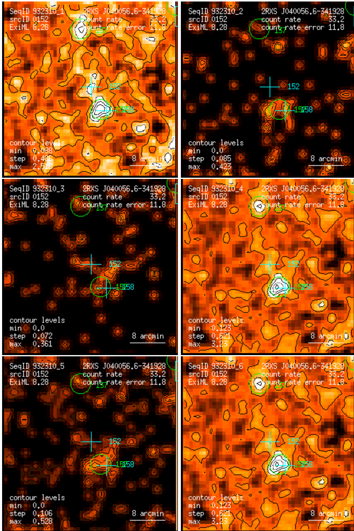
Figure 152: RASS 932310: detection 0152: band rate images, Gaussian filter: (1) PSPC channels 11 – 41, (2) 52 – 90, (3) 91 – 201, (4) 11 – 235, (5) 52 – 201, (6) 11 – 201. Broad band rates in counts/ks. Band rate contour levels in counts/ks/arcmin 2 .
