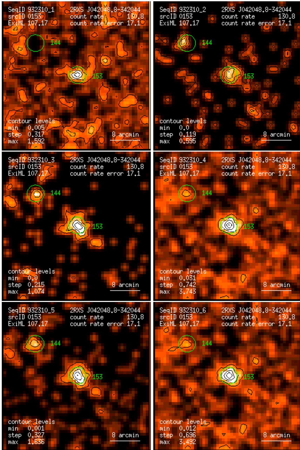
Figure 153: RASS 932310: detection 0153: band rate images, Gaussian filter: (1) PSPC channels 11 – 41, (2) 52 – 90, (3) 91 – 201, (4) 11 – 235, (5) 52 – 201, (6) 11 – 201. Broad band rates in counts/ks. Band rate contour levels in counts/ks/arcmin 2 .
