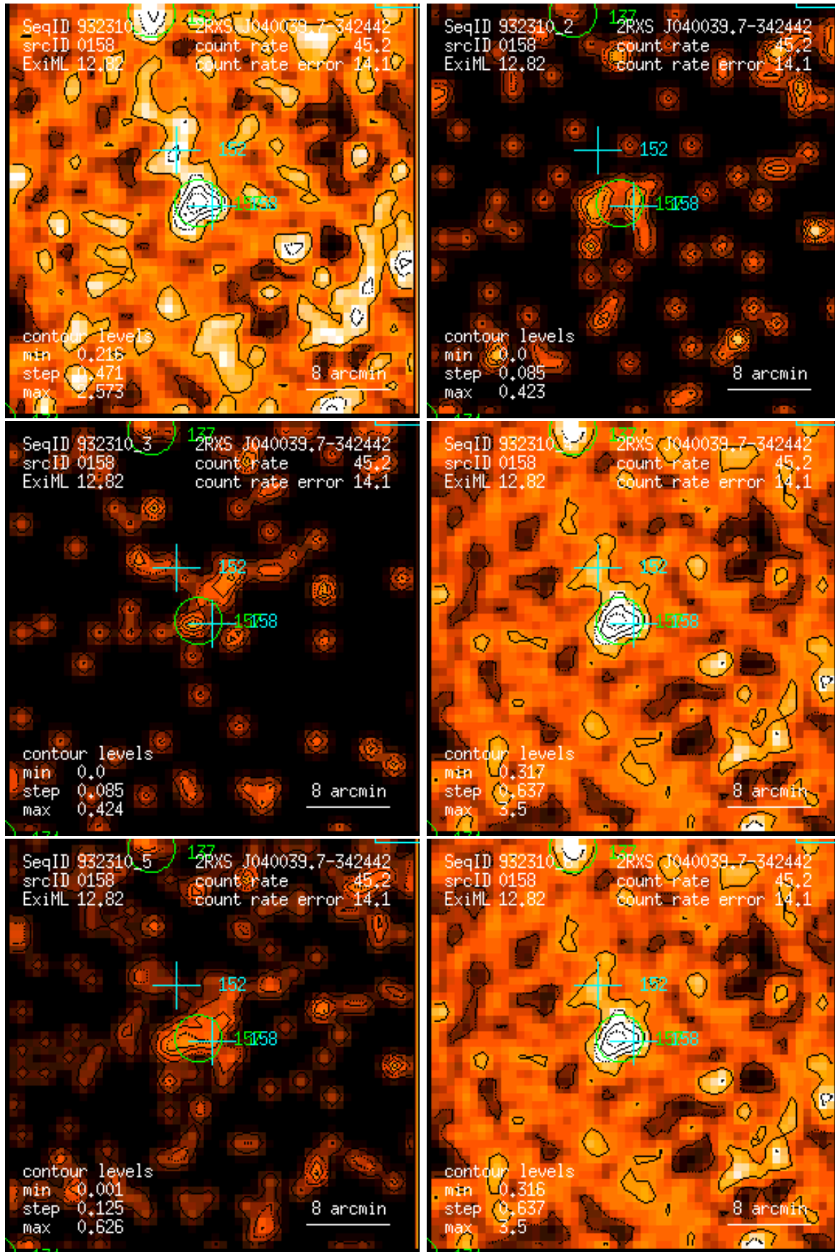
Figure 158: RASS 932310: detection 0158: band rate images, Gaussian filter: (1) PSPC channels 11 – 41, (2) 52 – 90, (3) 91 – 201, (4) 11 – 235, (5) 52 – 201, (6) 11 – 201. Broad band rates in counts/ks. Band rate contour levels in counts/ks/arcmin 2 .
