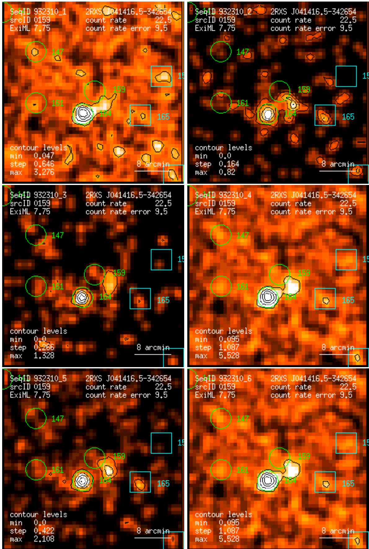
Figure 159: RASS 932310: detection 0159: band rate images, Gaussian filter: (1) PSPC channels 11 – 41, (2) 52 – 90, (3) 91 – 201, (4) 11 – 235, (5) 52 – 201, (6) 11 – 201. Broad band rates in counts/ks. Band rate contour levels in counts/ks/arcmin 2 .
