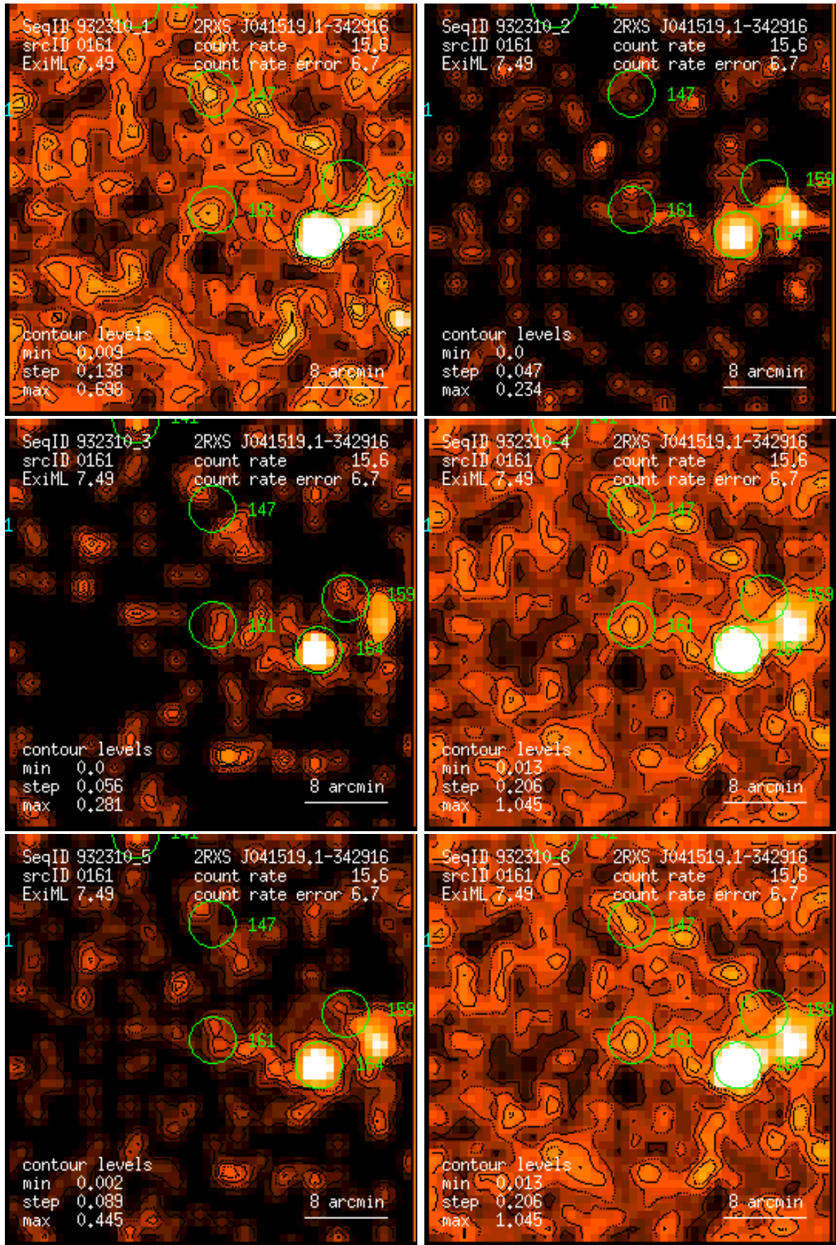
Figure 161: RASS 932310: detection 0161: band rate images, Gaussian filter: (1) PSPC channels 11 – 41, (2) 52 – 90, (3) 91 – 201, (4) 11 – 235, (5) 52 – 201, (6) 11 – 201. Broad band rates in counts/ks. Band rate contour levels in counts/ks/arcmin 2 .
