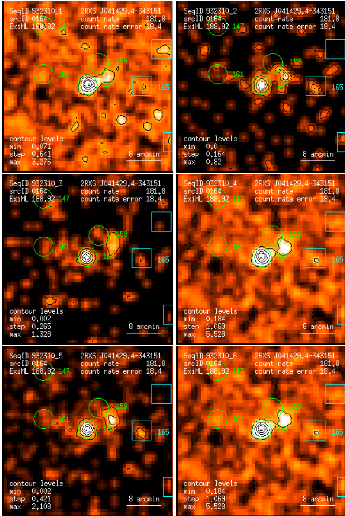
Figure 164: RASS 932310: detection 0164: band rate images, Gaussian filter: (1) PSPC channels 11 – 41, (2) 52 – 90, (3) 91 – 201, (4) 11 – 235, (5) 52 – 201, (6) 11 – 201. Broad band rates in counts/ks. Band rate contour levels in counts/ks/arcmin 2 .
