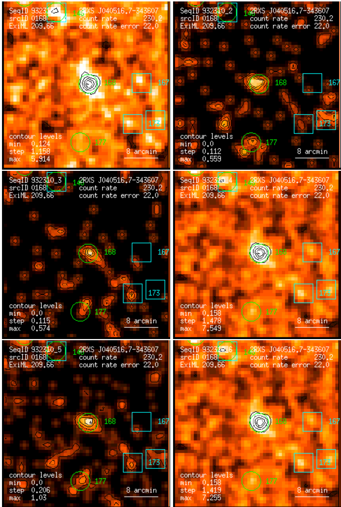
Figure 168: RASS 932310: detection 0168: band rate images, Gaussian filter: (1) PSPC channels 11 – 41, (2) 52 – 90, (3) 91 – 201, (4) 11 – 235, (5) 52 – 201, (6) 11 – 201. Broad band rates in counts/ks. Band rate contour levels in counts/ks/arcmin 2 .
