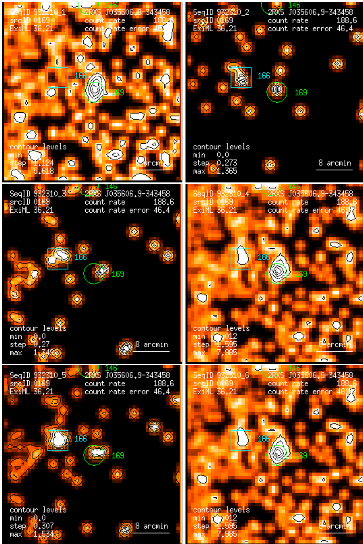
Figure 169: RASS 932310: detection 0169: band rate images, Gaussian filter: (1) PSPC channels 11 – 41, (2) 52 – 90, (3) 91 – 201, (4) 11 – 235, (5) 52 – 201, (6) 11 – 201. Broad band rates in counts/ks. Band rate contour levels in counts/ks/arcmin 2 .
