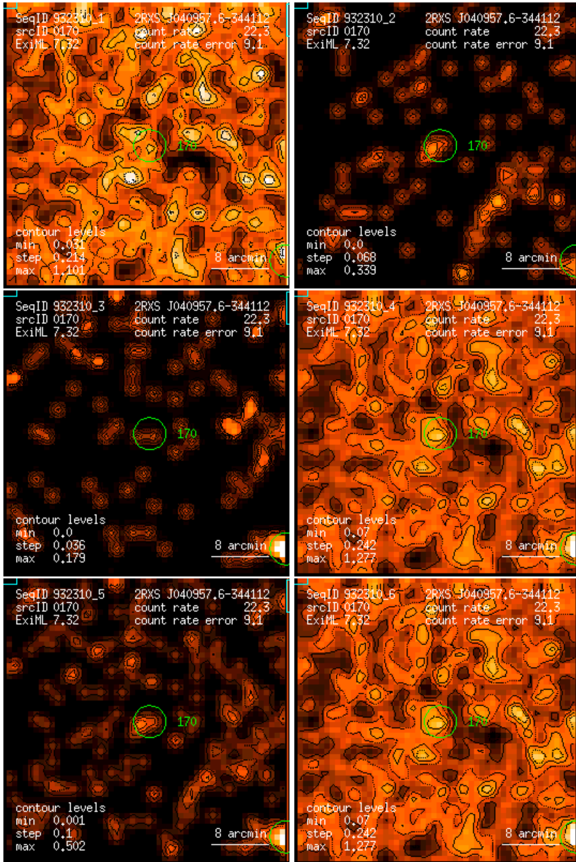
Figure 170: RASS 932310: detection 0170: band rate images, Gaussian filter: (1) PSPC channels 11 – 41, (2) 52 – 90, (3) 91 – 201, (4) 11 – 235, (5) 52 – 201, (6) 11 – 201. Broad band rates in counts/ks. Band rate contour levels in counts/ks/arcmin 2 .
