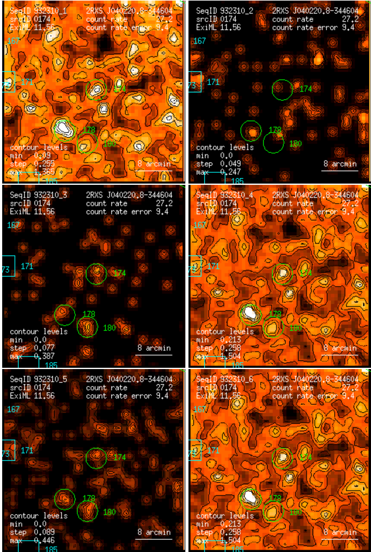
Figure 174: RASS 932310: detection 0174: band rate images, Gaussian filter: (1) PSPC channels 11 – 41, (2) 52 – 90, (3) 91 – 201, (4) 11 – 235, (5) 52 – 201, (6) 11 – 201. Broad band rates in counts/ks. Band rate contour levels in counts/ks/arcmin 2 .
