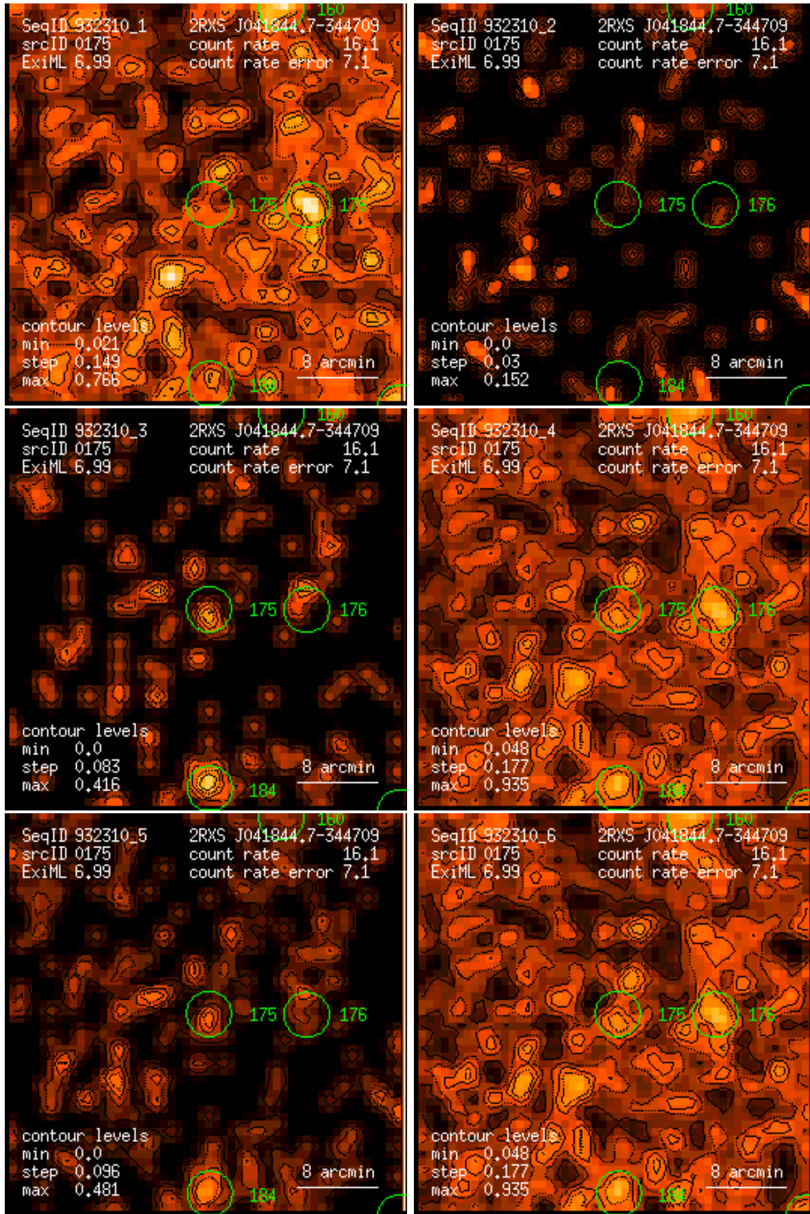
Figure 175: RASS 932310: detection 0175: band rate images, Gaussian filter: (1) PSPC channels 11 – 41, (2) 52 – 90, (3) 91 – 201, (4) 11 – 235, (5) 52 – 201, (6) 11 – 201. Broad band rates in counts/ks. Band rate contour levels in counts/ks/arcmin 2 .
