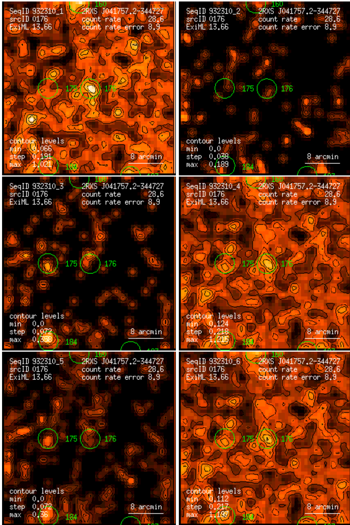
Figure 176: RASS 932310: detection 0176: band rate images, Gaussian filter: (1) PSPC channels 11 – 41, (2) 52 – 90, (3) 91 – 201, (4) 11 – 235, (5) 52 – 201, (6) 11 – 201. Broad band rates in counts/ks. Band rate contour levels in counts/ks/arcmin 2 .
