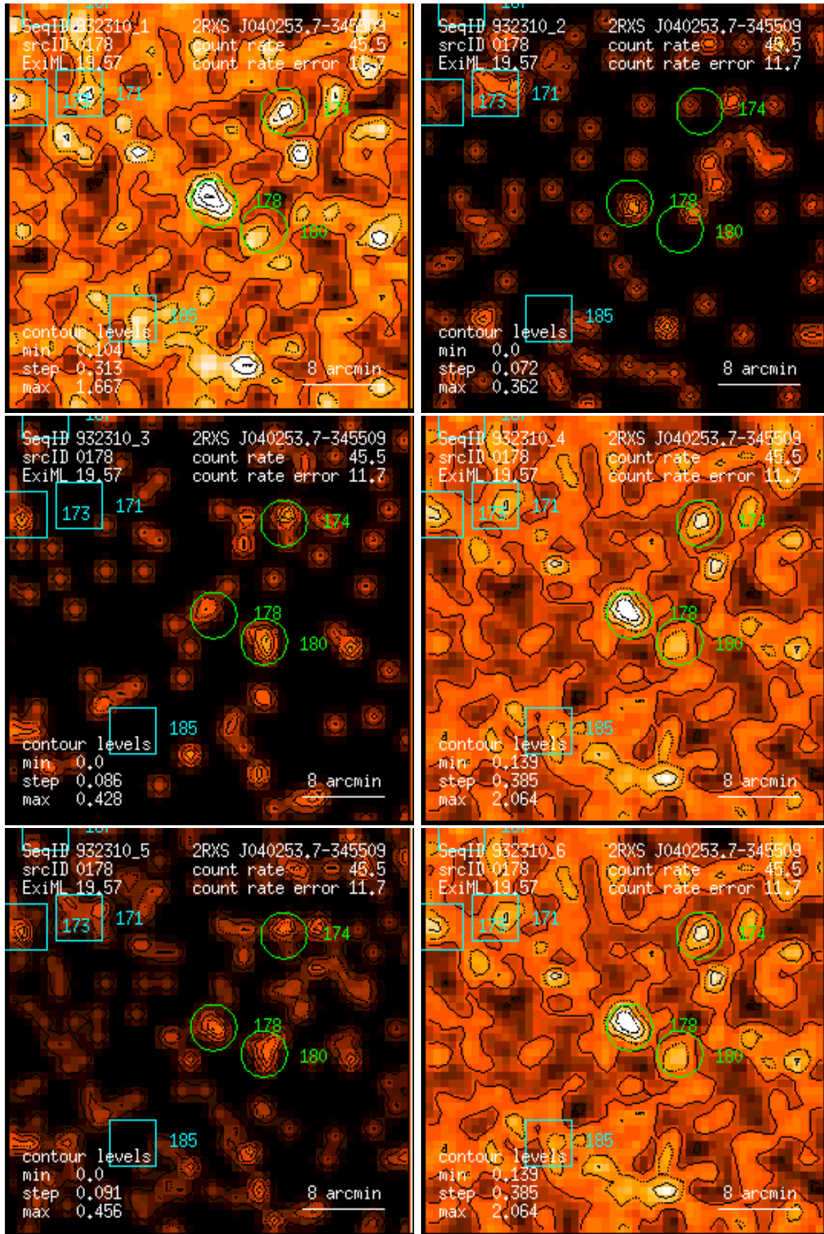
Figure 178: RASS 932310: detection 0178: band rate images, Gaussian filter: (1) PSPC channels 11 – 41, (2) 52 – 90, (3) 91 – 201, (4) 11 – 235, (5) 52 – 201, (6) 11 – 201. Broad band rates in counts/ks. Band rate contour levels in counts/ks/arcmin 2 .
