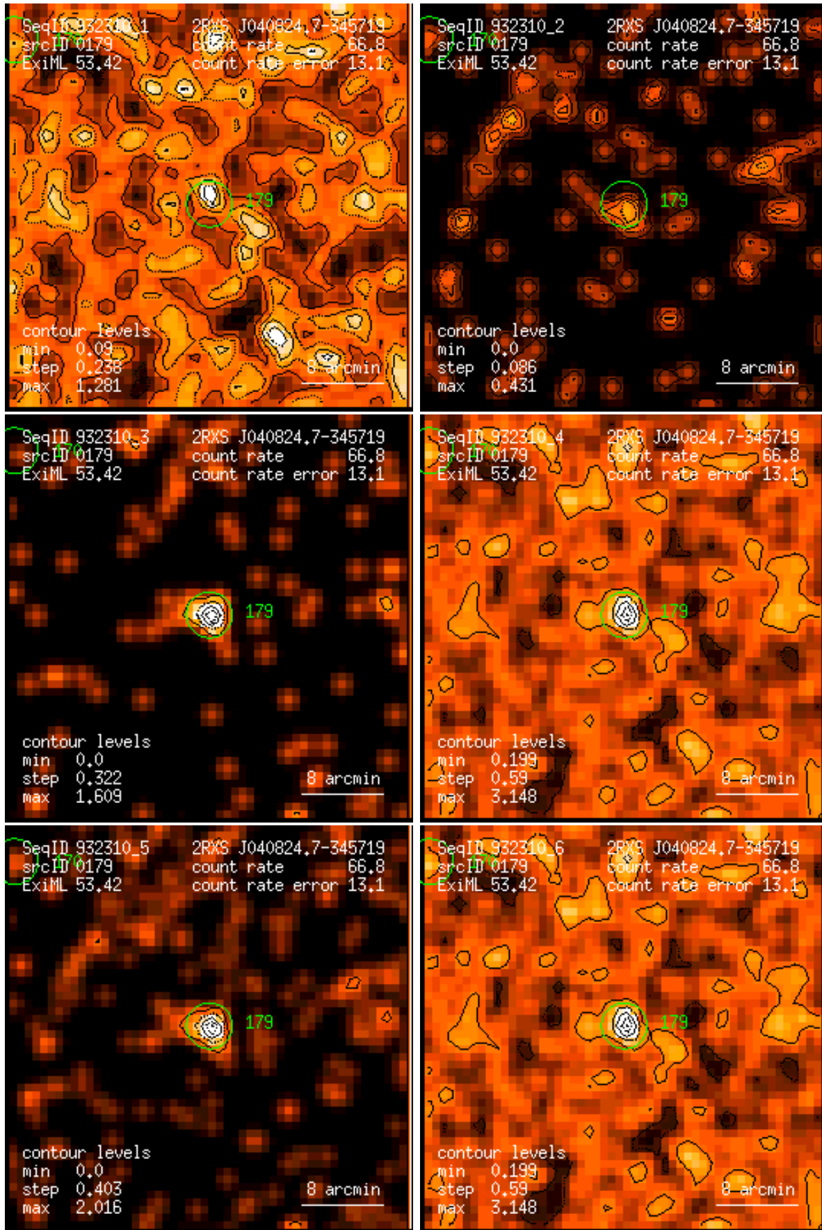
Figure 179: RASS 932310: detection 0179: band rate images, Gaussian filter: (1) PSPC channels 11 – 41, (2) 52 – 90, (3) 91 – 201, (4) 11 – 235, (5) 52 – 201, (6) 11 – 201. Broad band rates in counts/ks. Band rate contour levels in counts/ks/arcmin 2 .
