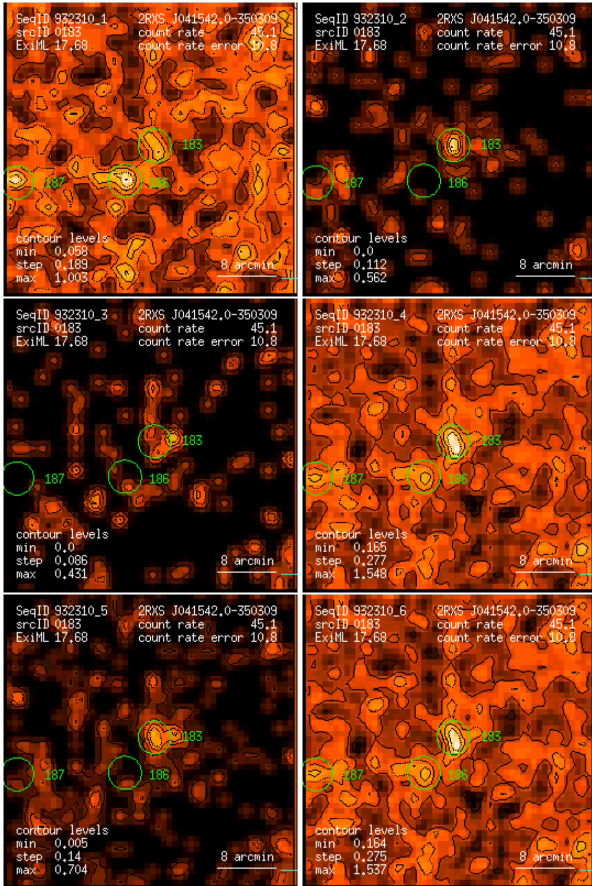
Figure 183: RASS 932310: detection 0183: band rate images, Gaussian filter: (1) PSPC channels 11 – 41, (2) 52 – 90, (3) 91 – 201, (4) 11 – 235, (5) 52 – 201, (6) 11 – 201. Broad band rates in counts/ks. Band rate contour levels in counts/ks/arcmin 2 .
