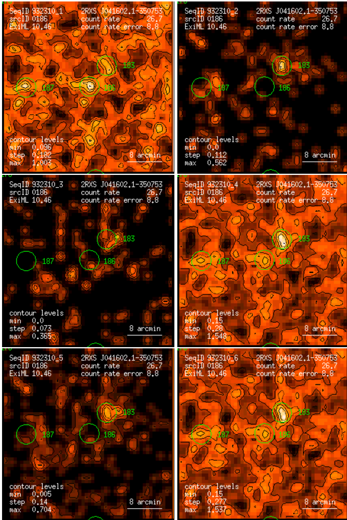
Figure 186: RASS 932310: detection 0186: band rate images, Gaussian filter: (1) PSPC channels 11 – 41, (2) 52 – 90, (3) 91 – 201, (4) 11 – 235, (5) 52 – 201, (6) 11 – 201. Broad band rates in counts/ks. Band rate contour levels in counts/ks/arcmin 2 .
