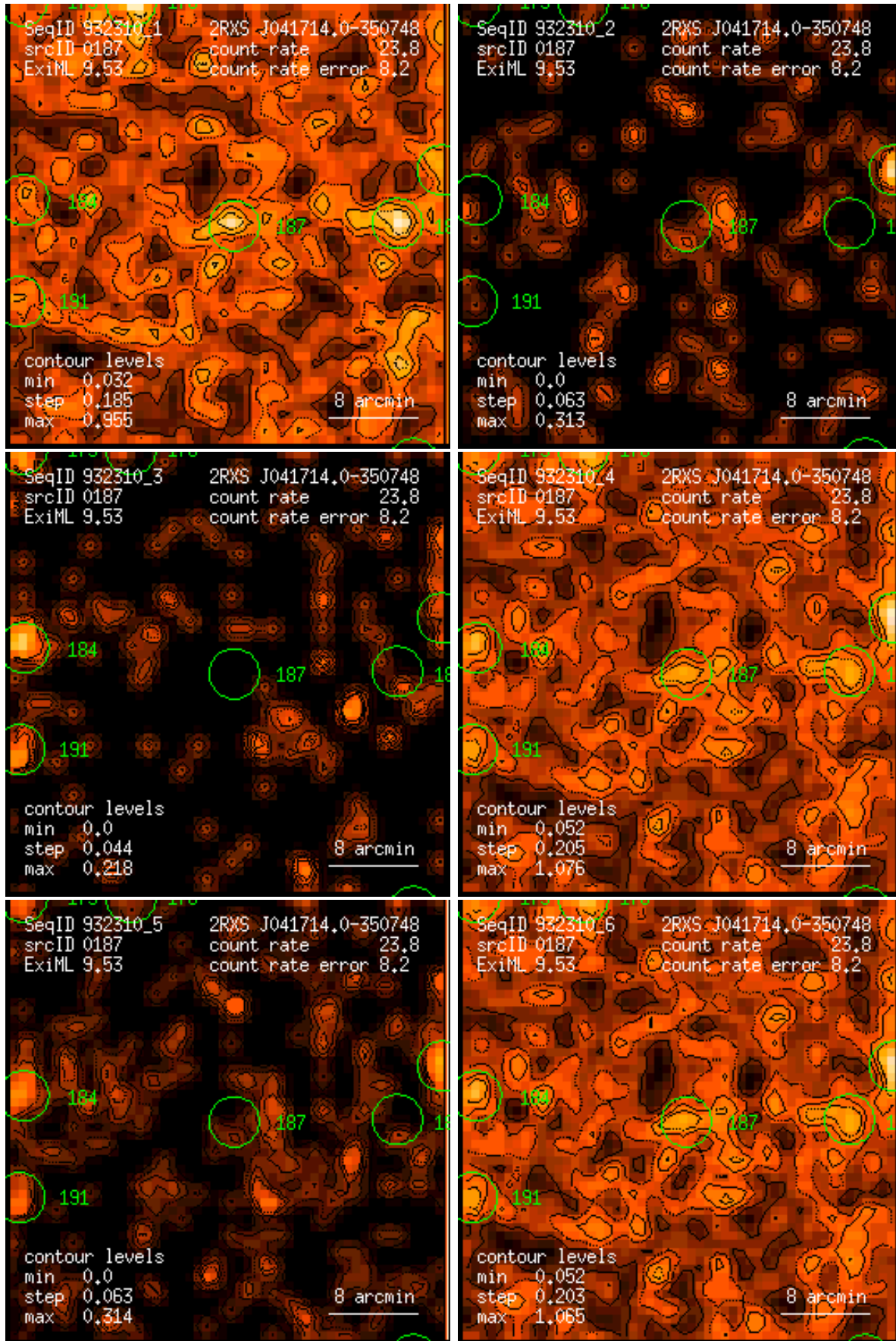
Figure 187: RASS 932310: detection 0187: band rate images, Gaussian filter: (1) PSPC channels 11 – 41, (2) 52 – 90, (3) 91 – 201, (4) 11 – 235, (5) 52 – 201, (6) 11 – 201. Broad band rates in counts/ks. Band rate contour levels in counts/ks/arcmin 2 .
