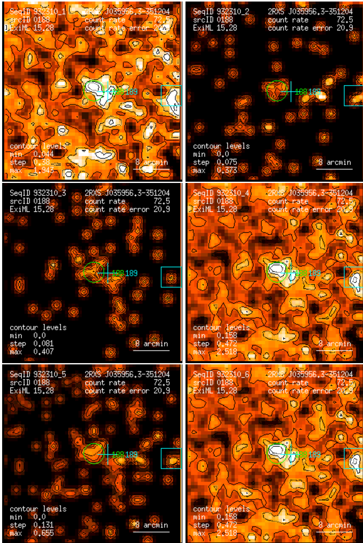
Figure 188: RASS 932310: detection 0188: band rate images, Gaussian filter: (1) PSPC channels 11 – 41, (2) 52 – 90, (3) 91 – 201, (4) 11 – 235, (5) 52 – 201, (6) 11 – 201. Broad band rates in counts/ks. Band rate contour levels in counts/ks/arcmin 2 .
