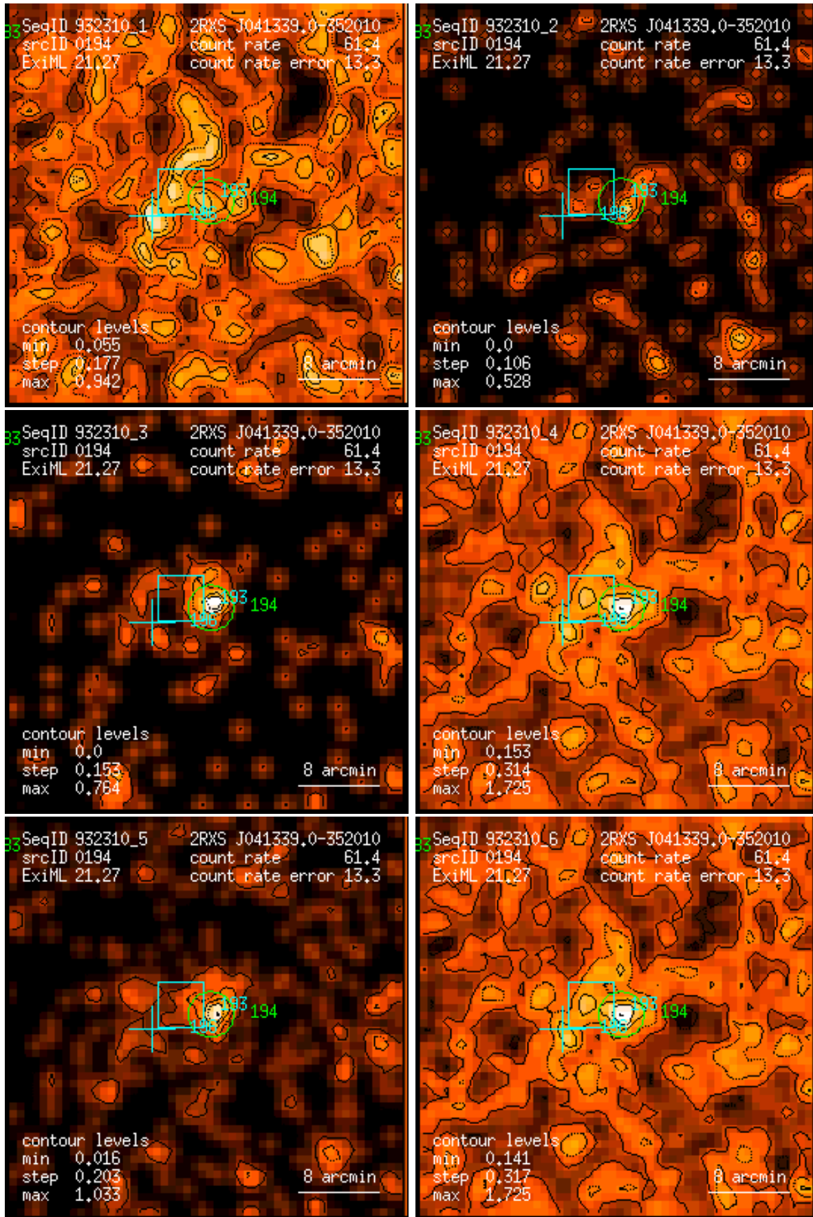
Figure 194: RASS 932310: detection 0194: band rate images, Gaussian filter: (1) PSPC channels 11 – 41, (2) 52 – 90, (3) 91 – 201, (4) 11 – 235, (5) 52 – 201, (6) 11 – 201. Broad band rates in counts/ks. Band rate contour levels in counts/ks/arcmin 2 .
