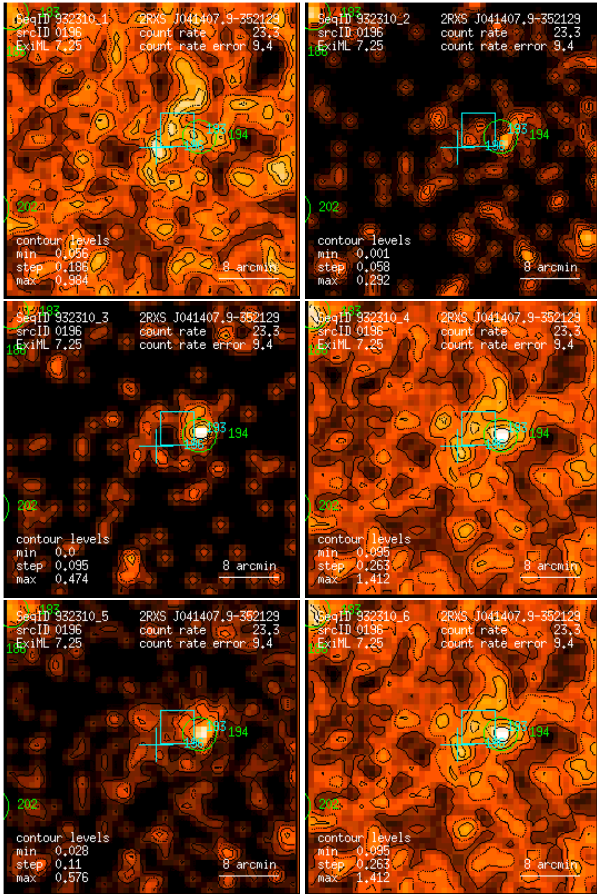
Figure 196: RASS 932310: detection 0196: band rate images, Gaussian filter: (1) PSPC channels 11 – 41, (2) 52 – 90, (3) 91 – 201, (4) 11 – 235, (5) 52 – 201, (6) 11 – 201. Broad band rates in counts/ks. Band rate contour levels in counts/ks/arcmin 2 .
