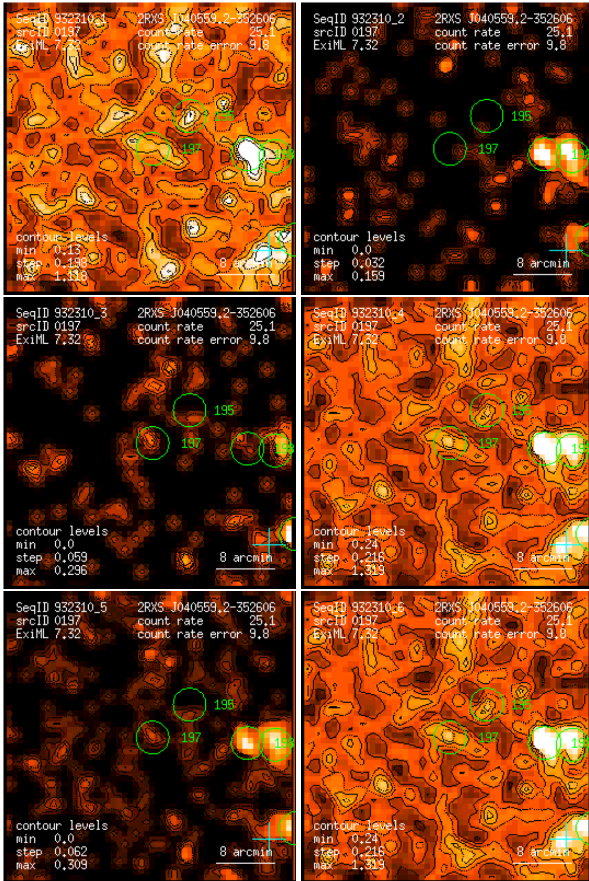
Figure 197: RASS 932310: detection 0197: band rate images, Gaussian filter: (1) PSPC channels 11 – 41, (2) 52 – 90, (3) 91 – 201, (4) 11 – 235, (5) 52 – 201, (6) 11 – 201. Broad band rates in counts/ks. Band rate contour levels in counts/ks/arcmin 2 .
