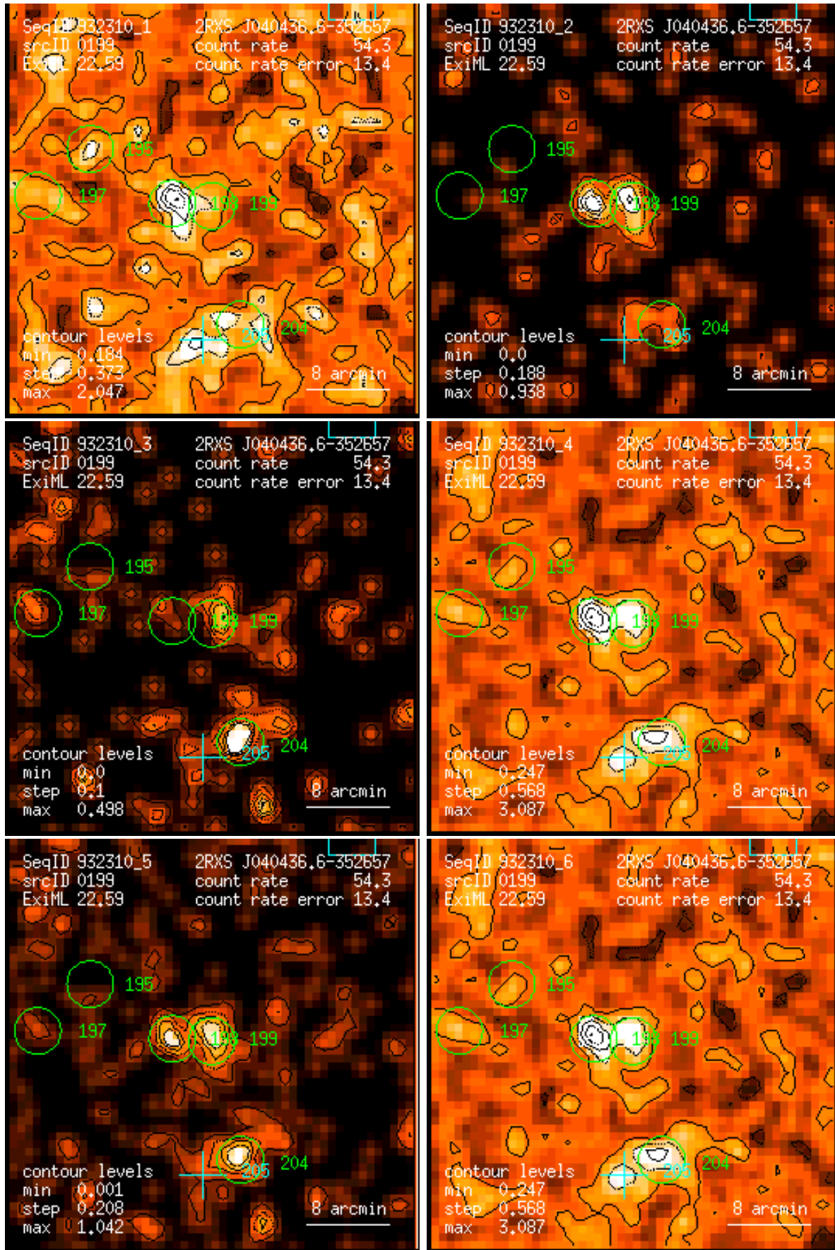
Figure 199: RASS 932310: detection 0199: band rate images, Gaussian filter: (1) PSPC channels 11 – 41, (2) 52 – 90, (3) 91 – 201, (4) 11 – 235, (5) 52 – 201, (6) 11 – 201. Broad band rates in counts/ks. Band rate contour levels in counts/ks/arcmin 2 .
