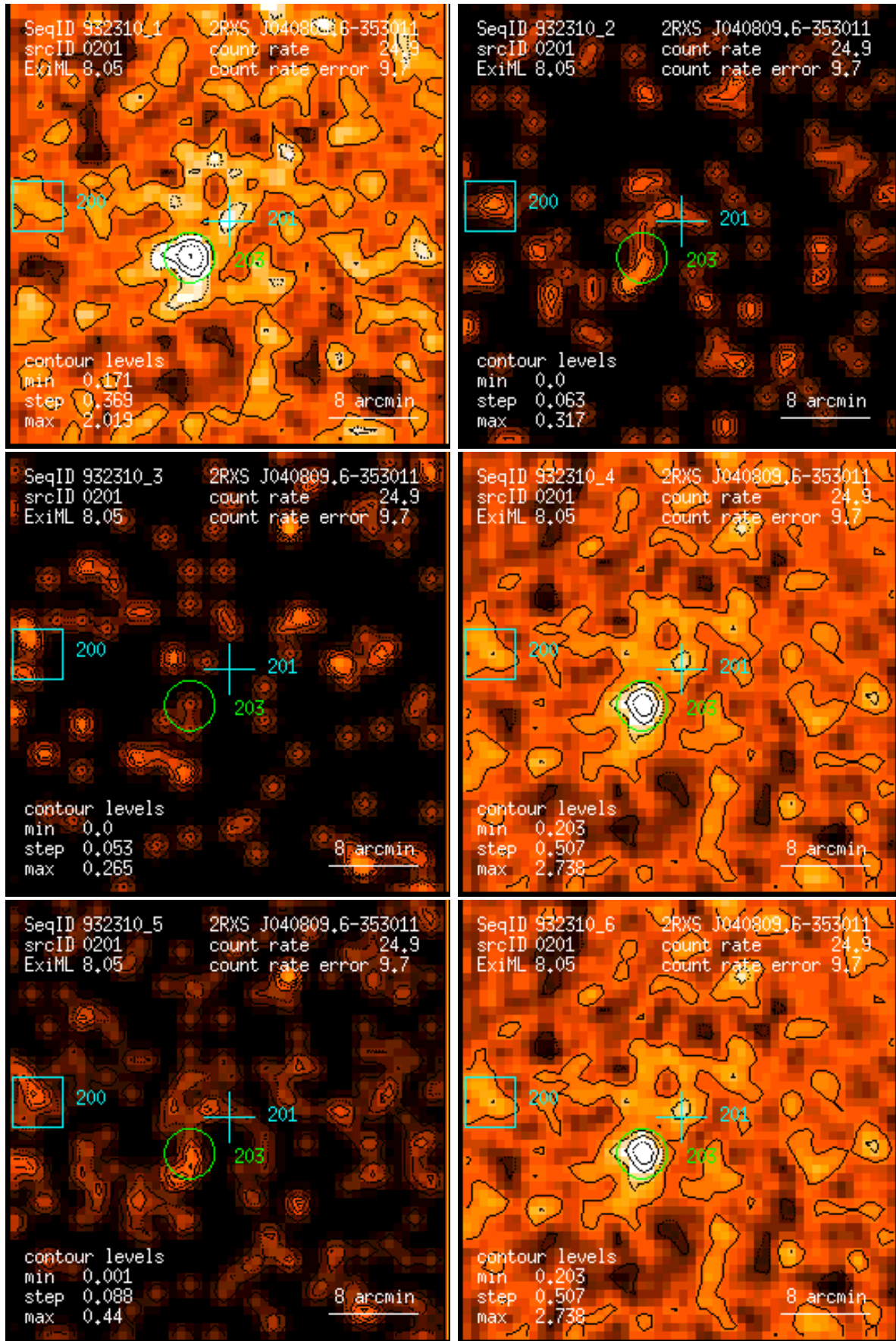
Figure 201: RASS 932310: detection 0201: band rate images, Gaussian filter: (1) PSPC channels 11 – 41, (2) 52 – 90, (3) 91 – 201, (4) 11 – 235, (5) 52 – 201, (6) 11 – 201. Broad band rates in counts/ks. Band rate contour levels in counts/ks/arcmin 2 .
