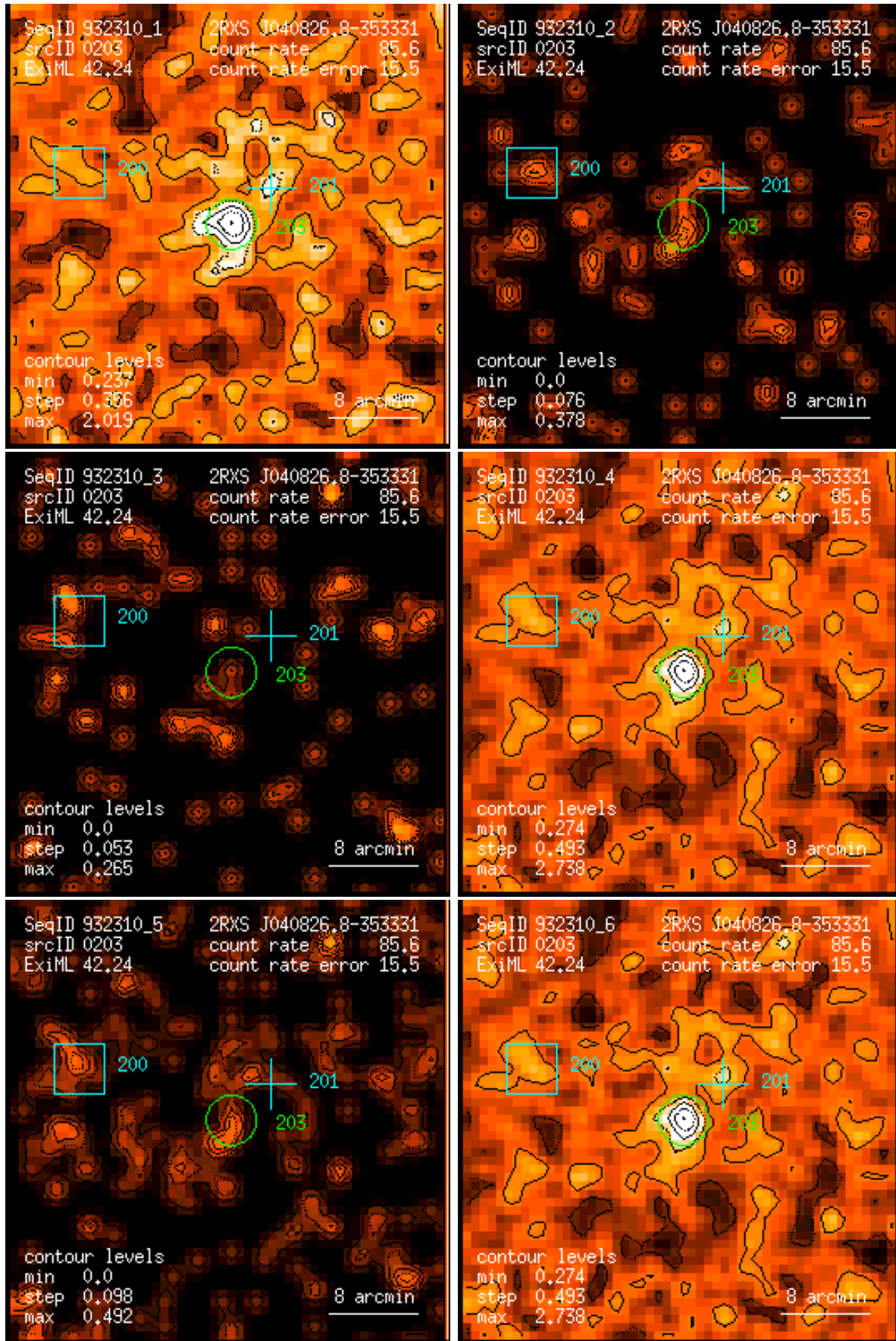
Figure 203: RASS 932310: detection 0203: band rate images, Gaussian filter: (1) PSPC channels 11 – 41, (2) 52 – 90, (3) 91 – 201, (4) 11 – 235, (5) 52 – 201, (6) 11 – 201. Broad band rates in counts/ks. Band rate contour levels in counts/ks/arcmin 2 .
