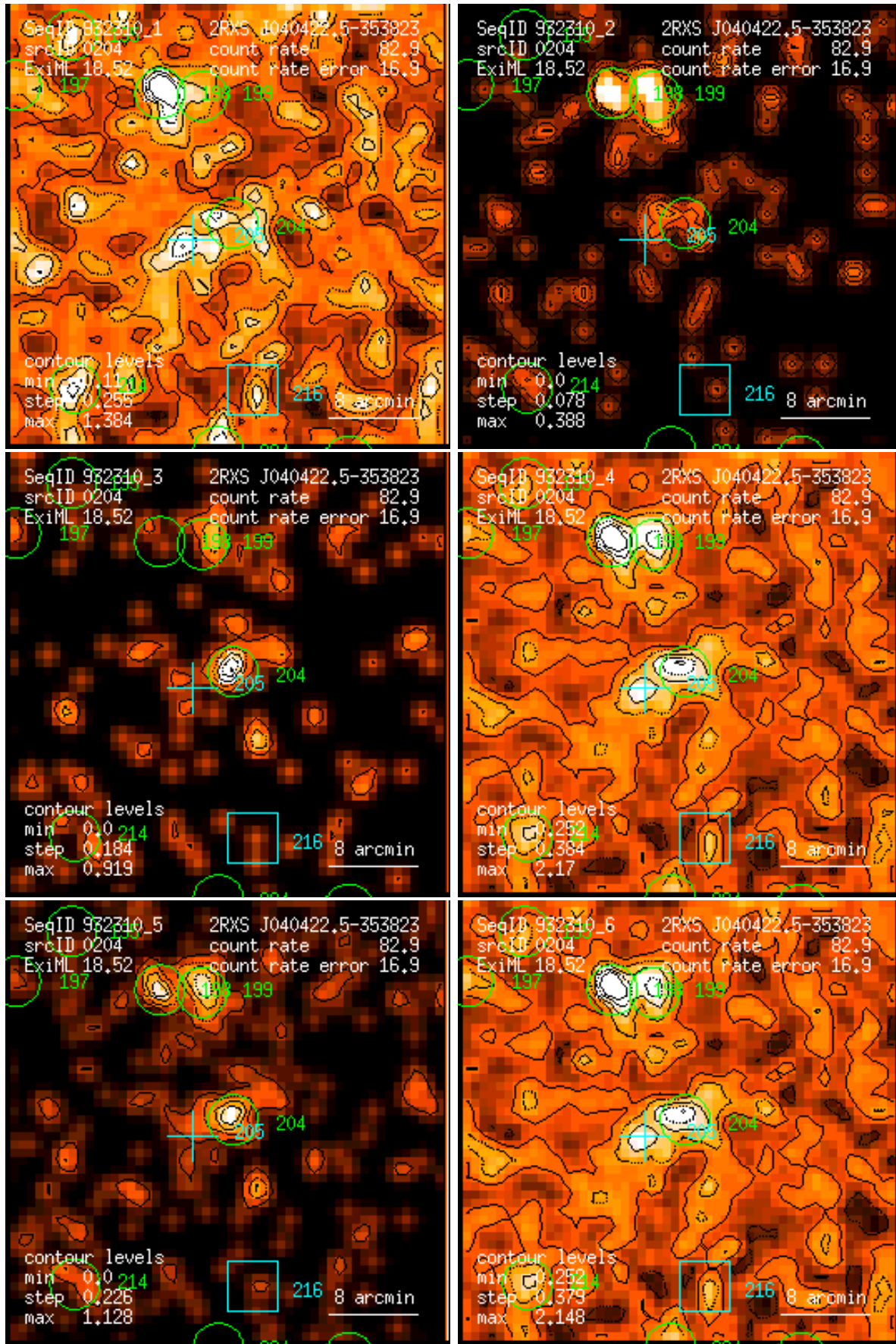
Figure 204: RASS 932310: detection 0204: band rate images, Gaussian filter: (1) PSPC channels 11 – 41, (2) 52 – 90, (3) 91 – 201, (4) 11 – 235, (5) 52 – 201, (6) 11 – 201. Broad band rates in counts/ks. Band rate contour levels in counts/ks/arcmin 2 .
