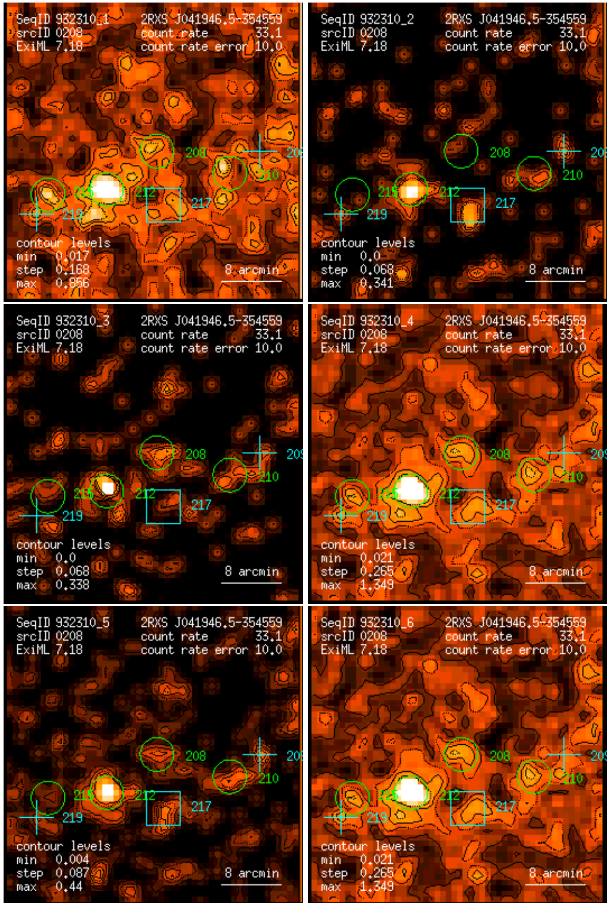
Figure 208: RASS 932310: detection 0208: band rate images, Gaussian filter: (1) PSPC channels 11 – 41, (2) 52 – 90, (3) 91 – 201, (4) 11 – 235, (5) 52 – 201, (6) 11 – 201. Broad band rates in counts/ks. Band rate contour levels in counts/ks/arcmin 2 .
