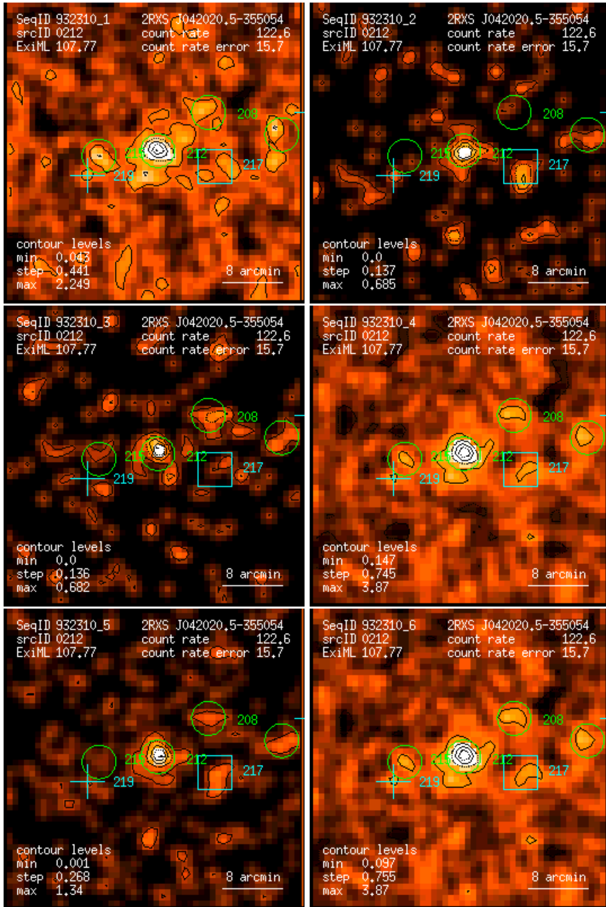
Figure 212: RASS 932310: detection 0212: band rate images, Gaussian filter: (1) PSPC channels 11 – 41, (2) 52 – 90, (3) 91 – 201, (4) 11 – 235, (5) 52 – 201, (6) 11 – 201. Broad band rates in counts/ks. Band rate contour levels in counts/ks/arcmin 2 .
