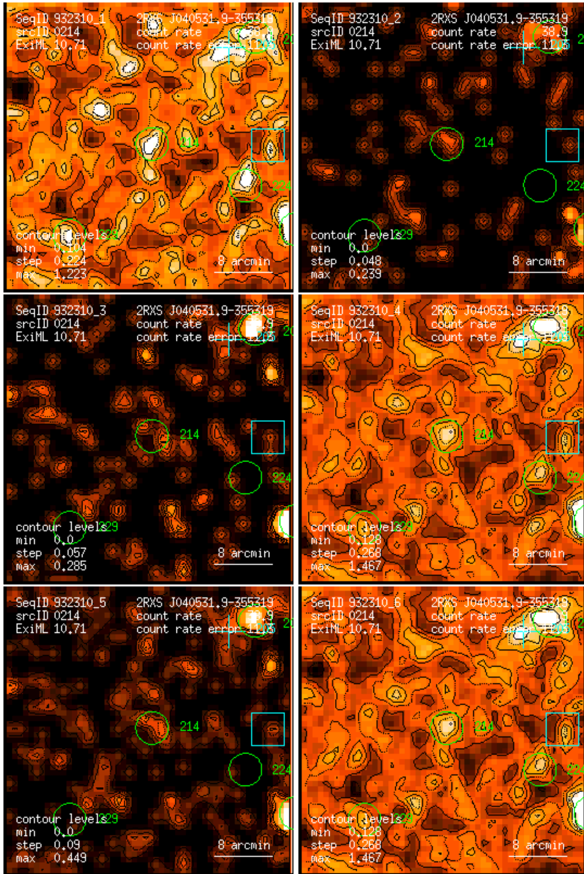
Figure 214: RASS 932310: detection 0214: band rate images, Gaussian filter: (1) PSPC channels 11 – 41, (2) 52 – 90, (3) 91 – 201, (4) 11 – 235, (5) 52 – 201, (6) 11 – 201. Broad band rates in counts/ks. Band rate contour levels in counts/ks/arcmin 2 .
