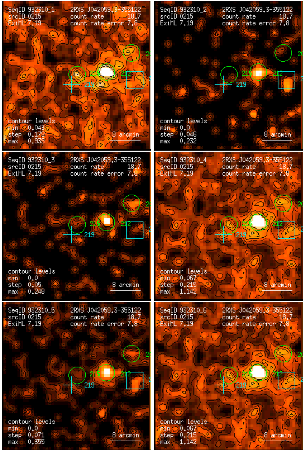
Figure 215: RASS 932310: detection 0215: band rate images, Gaussian filter: (1) PSPC channels 11 – 41, (2) 52 – 90, (3) 91 – 201, (4) 11 – 235, (5) 52 – 201, (6) 11 – 201. Broad band rates in counts/ks. Band rate contour levels in counts/ks/arcmin 2 .
