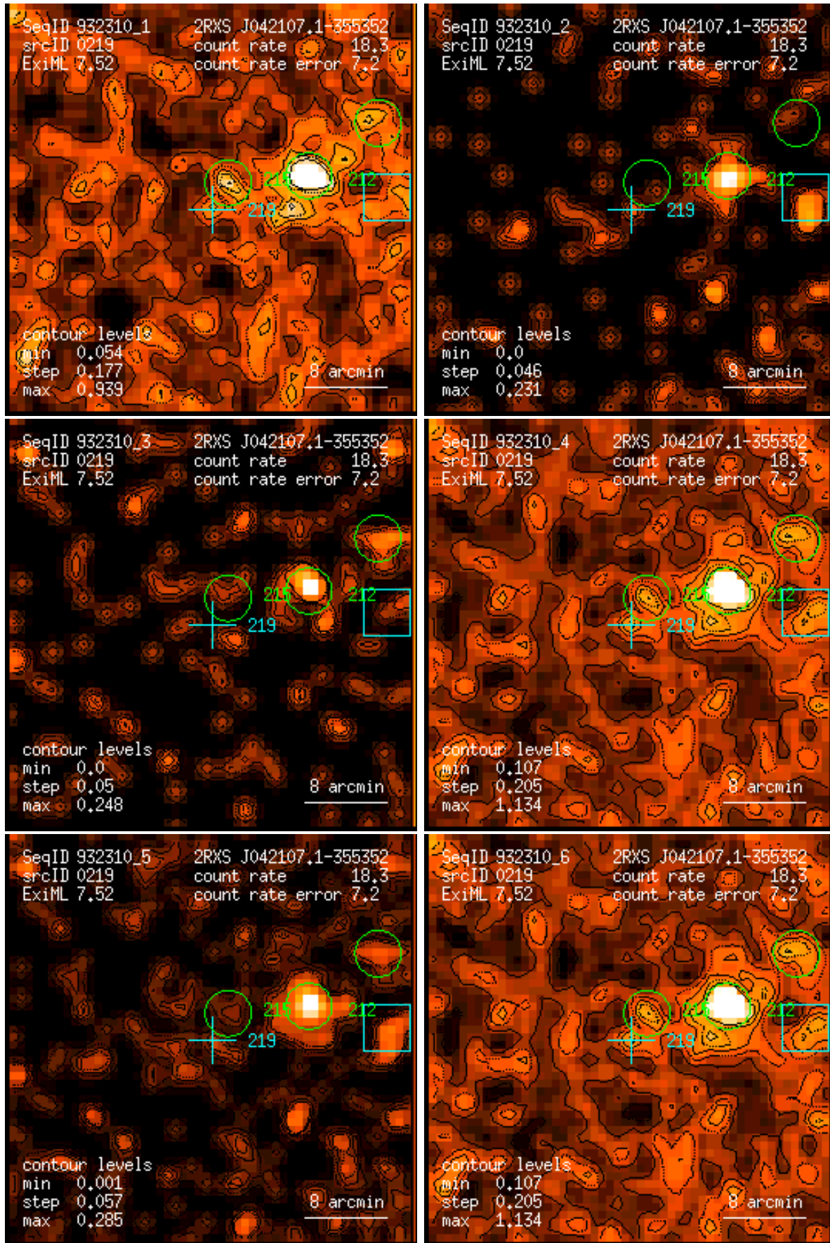
Figure 219: RASS 932310: detection 0219: band rate images, Gaussian filter: (1) PSPC channels 11 – 41, (2) 52 – 90, (3) 91 – 201, (4) 11 – 235, (5) 52 – 201, (6) 11 – 201. Broad band rates in counts/ks. Band rate contour levels in counts/ks/arcmin 2 .
