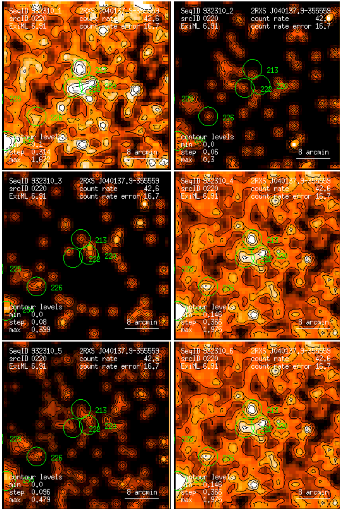
Figure 220: RASS 932310: detection 0220: band rate images, Gaussian filter: (1) PSPC channels 11 – 41, (2) 52 – 90, (3) 91 – 201, (4) 11 – 235, (5) 52 – 201, (6) 11 – 201. Broad band rates in counts/ks. Band rate contour levels in counts/ks/arcmin 2 .
