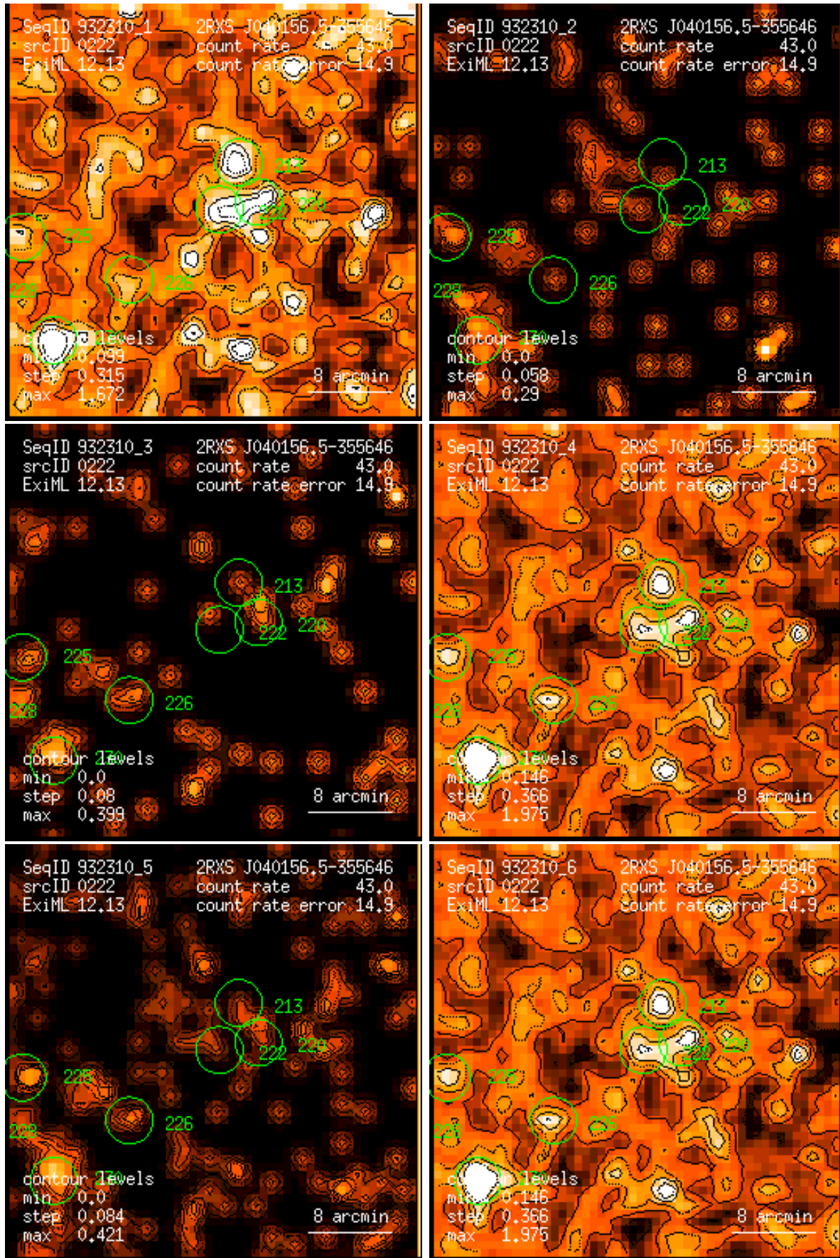
Figure 222: RASS 932310: detection 0222: band rate images, Gaussian filter: (1) PSPC channels 11 – 41, (2) 52 – 90, (3) 91 – 201, (4) 11 – 235, (5) 52 – 201, (6) 11 – 201. Broad band rates in counts/ks. Band rate contour levels in counts/ks/arcmin 2 .
