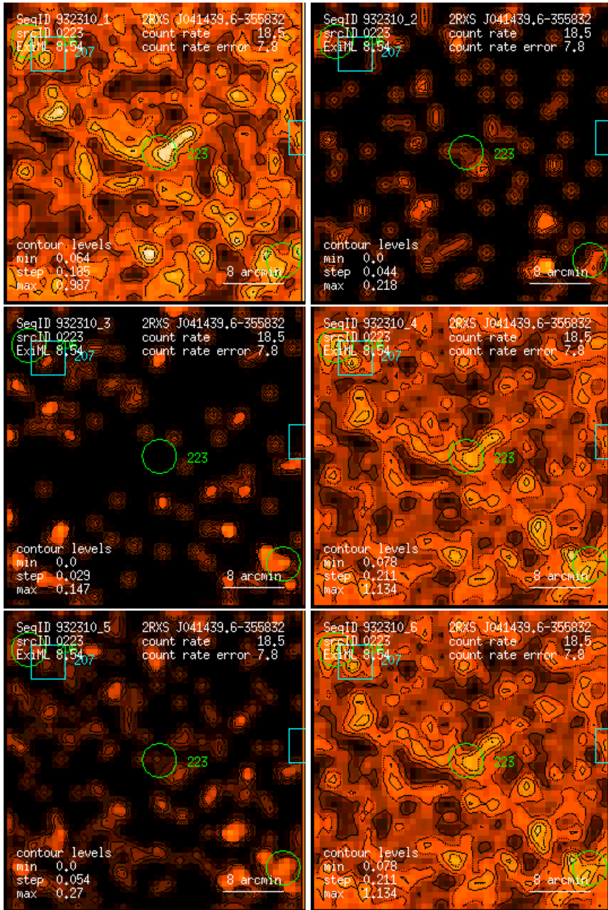
Figure 223: RASS 932310: detection 0223: band rate images, Gaussian filter: (1) PSPC channels 11 – 41, (2) 52 – 90, (3) 91 – 201, (4) 11 – 235, (5) 52 – 201, (6) 11 – 201. Broad band rates in counts/ks. Band rate contour levels in counts/ks/arcmin 2 .
