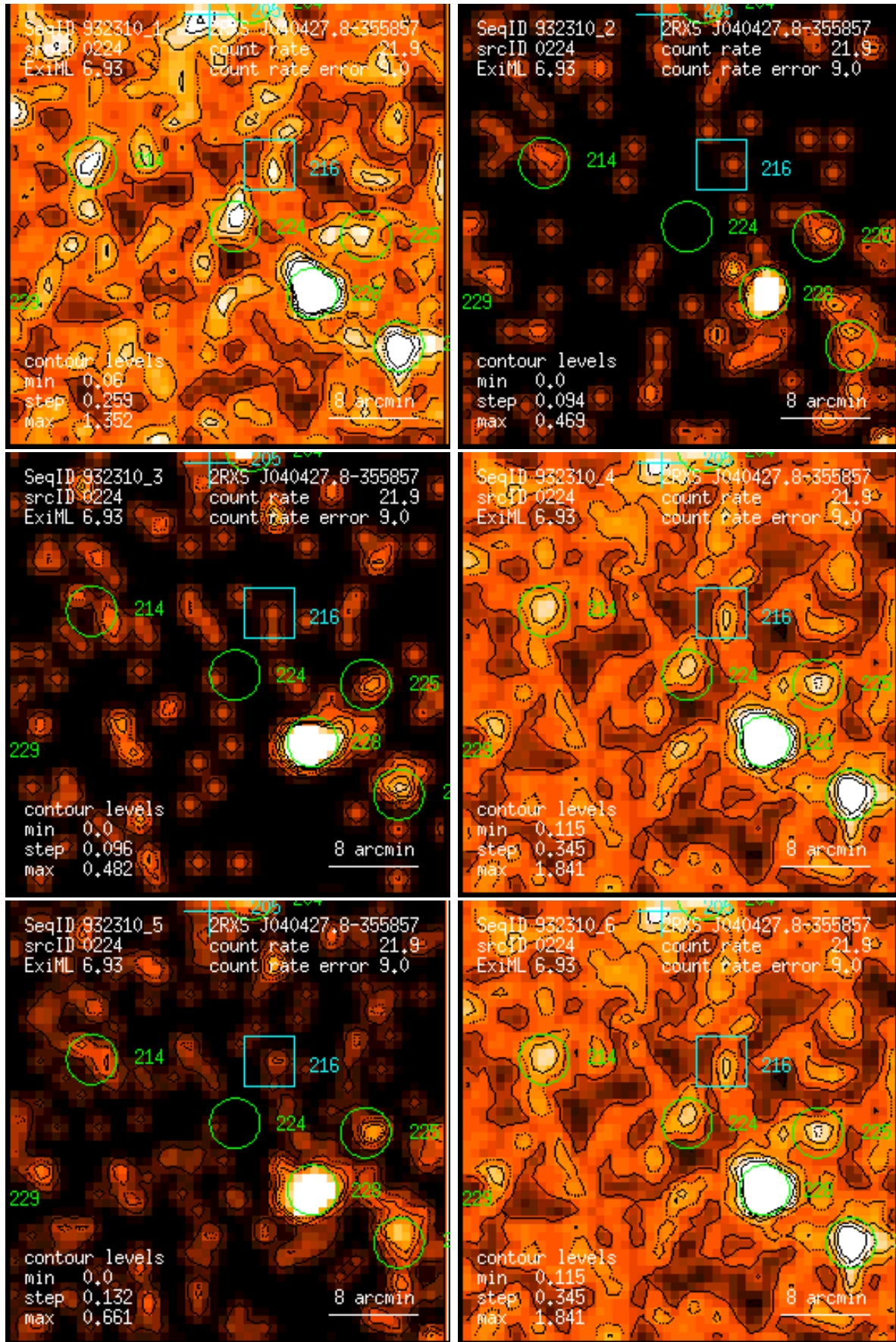
Figure 224: RASS 932310: detection 0224: band rate images, Gaussian filter: (1) PSPC channels 11 – 41, (2) 52 – 90, (3) 91 – 201, (4) 11 – 235, (5) 52 – 201, (6) 11 – 201. Broad band rates in counts/ks. Band rate contour levels in counts/ks/arcmin 2 .
