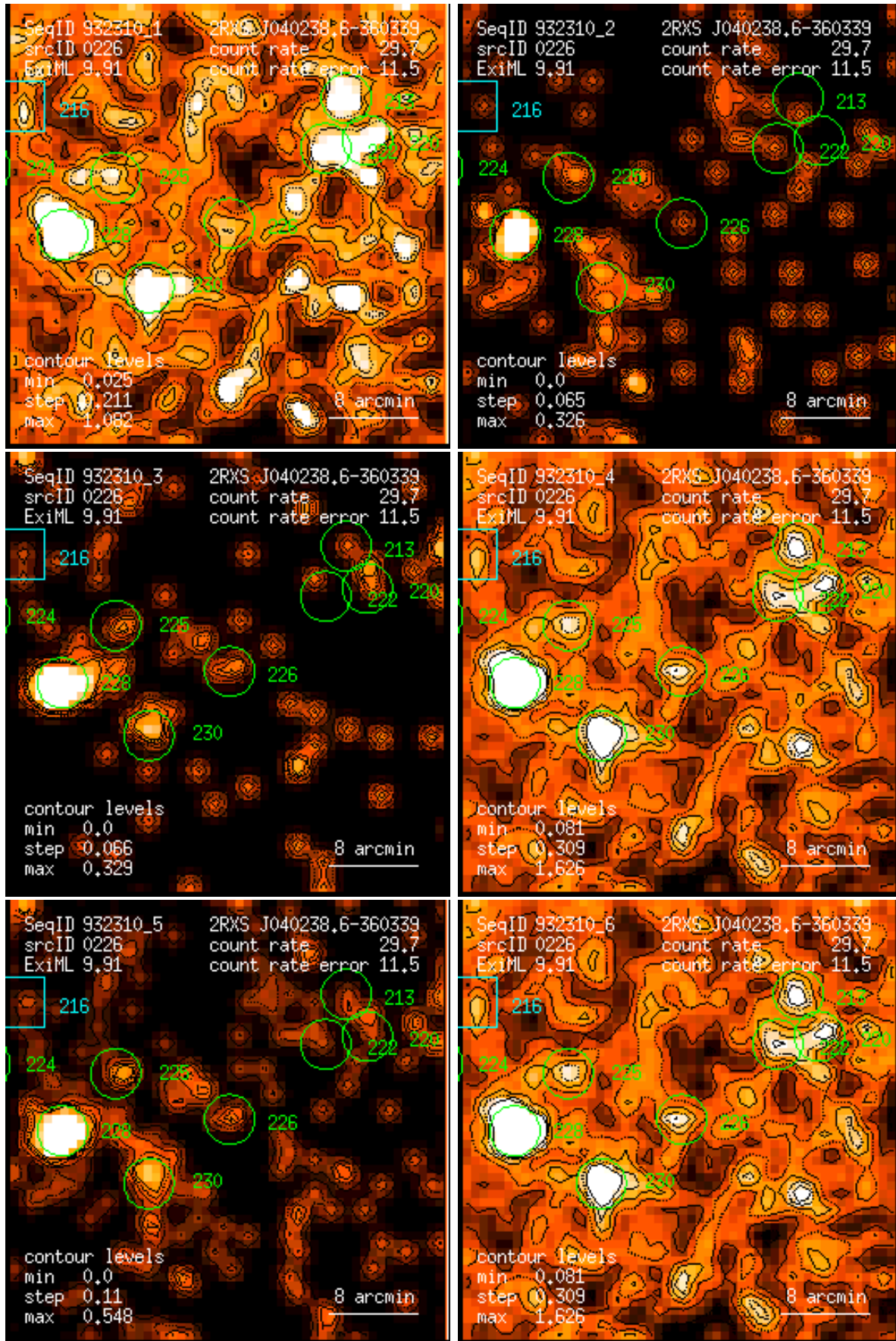
Figure 226: RASS 932310: detection 0226: band rate images, Gaussian filter: (1) PSPC channels 11 – 41, (2) 52 – 90, (3) 91 – 201, (4) 11 – 235, (5) 52 – 201, (6) 11 – 201. Broad band rates in counts/ks. Band rate contour levels in counts/ks/arcmin 2 .
