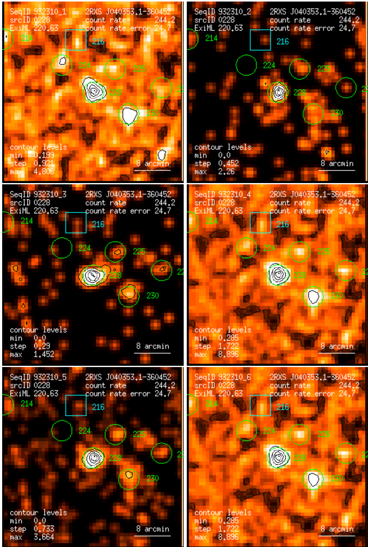
Figure 228: RASS 932310: detection 0228: band rate images, Gaussian filter: (1) PSPC channels 11 – 41, (2) 52 – 90, (3) 91 – 201, (4) 11 – 235, (5) 52 – 201, (6) 11 – 201. Broad band rates in counts/ks. Band rate contour levels in counts/ks/arcmin 2 .
