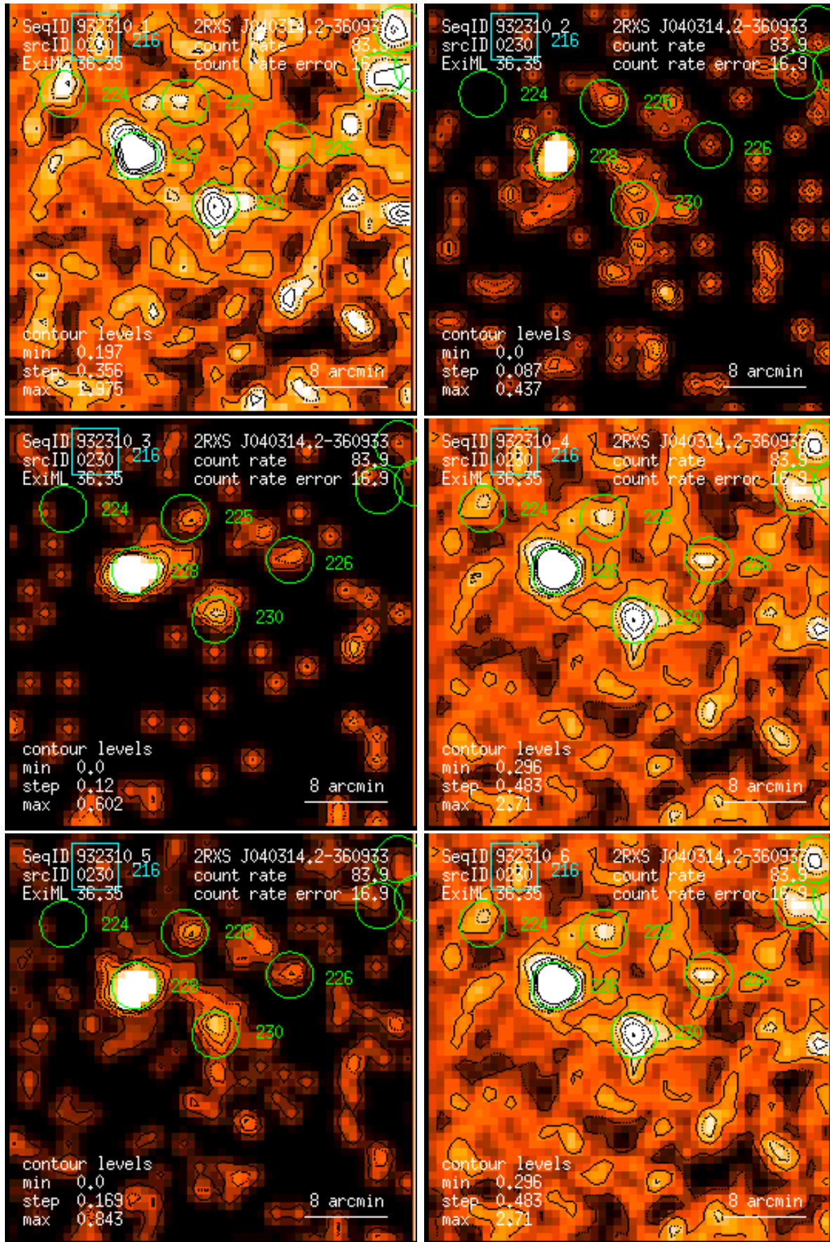
Figure 230: RASS 932310: detection 0230: band rate images, Gaussian filter: (1) PSPC channels 11 – 41, (2) 52 – 90, (3) 91 – 201, (4) 11 – 235, (5) 52 – 201, (6) 11 – 201. Broad band rates in counts/ks. Band rate contour levels in counts/ks/arcmin 2 .
