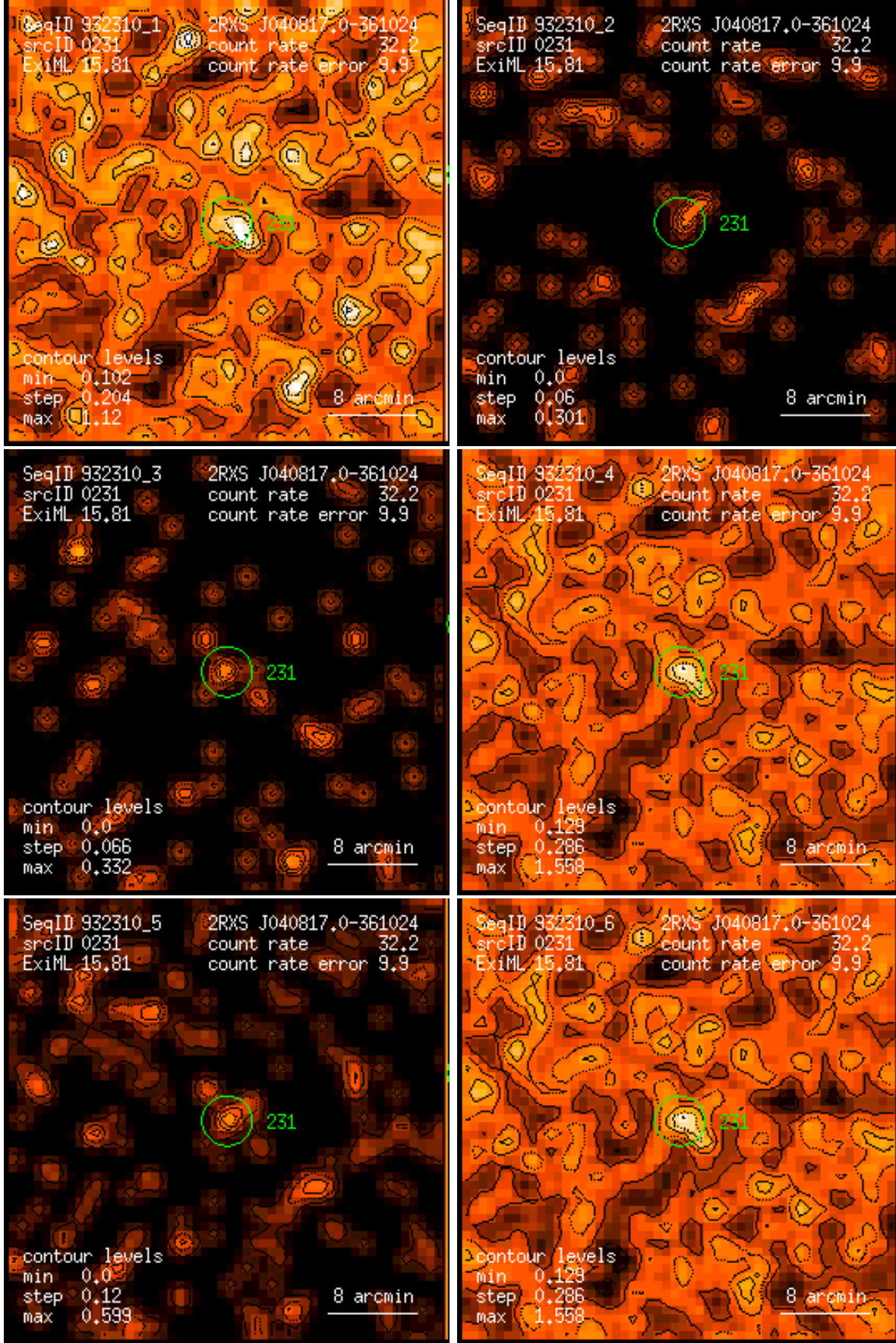
Figure 231: RASS 932310: detection 0231: band rate images, Gaussian filter: (1) PSPC channels 11 – 41, (2) 52 – 90, (3) 91 – 201, (4) 11 – 235, (5) 52 – 201, (6) 11 – 201. Broad band rates in counts/ks. Band rate contour levels in counts/ks/arcmin 2 .
