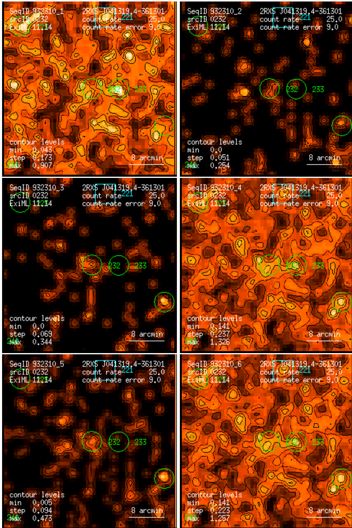
Figure 232: RASS 932310: detection 0232: band rate images, Gaussian filter: (1) PSPC channels 11 – 41, (2) 52 – 90, (3) 91 – 201, (4) 11 – 235, (5) 52 – 201, (6) 11 – 201. Broad band rates in counts/ks. Band rate contour levels in counts/ks/arcmin 2 .
