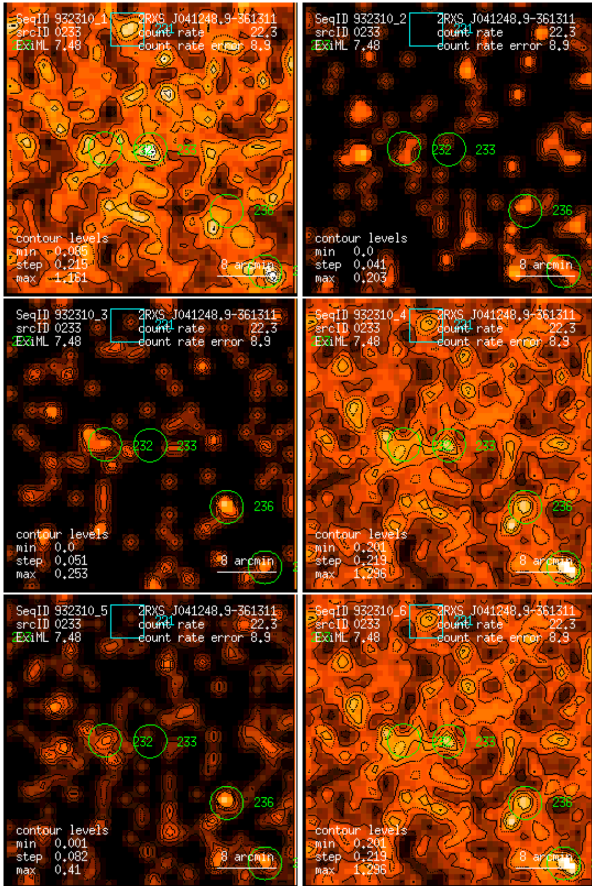
Figure 233: RASS 932310: detection 0233: band rate images, Gaussian filter: (1) PSPC channels 11 – 41, (2) 52 – 90, (3) 91 – 201, (4) 11 – 235, (5) 52 – 201, (6) 11 – 201. Broad band rates in counts/ks. Band rate contour levels in counts/ks/arcmin 2 .
