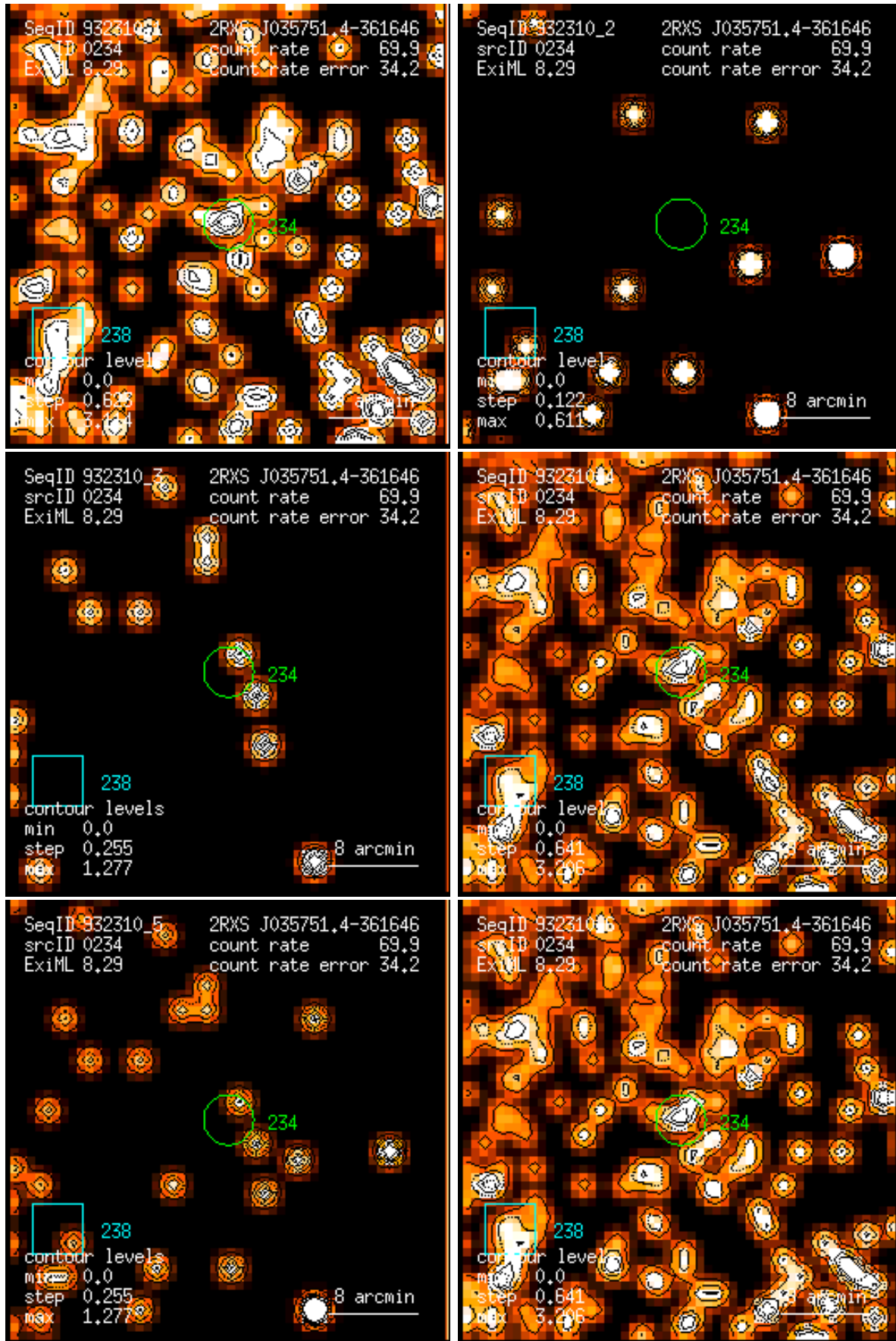
Figure 234: RASS 932310: detection 0234: band rate images, Gaussian filter: (1) PSPC channels 11 – 41, (2) 52 – 90, (3) 91 – 201, (4) 11 – 235, (5) 52 – 201, (6) 11 – 201. Broad band rates in counts/ks. Band rate contour levels in counts/ks/arcmin 2 .
