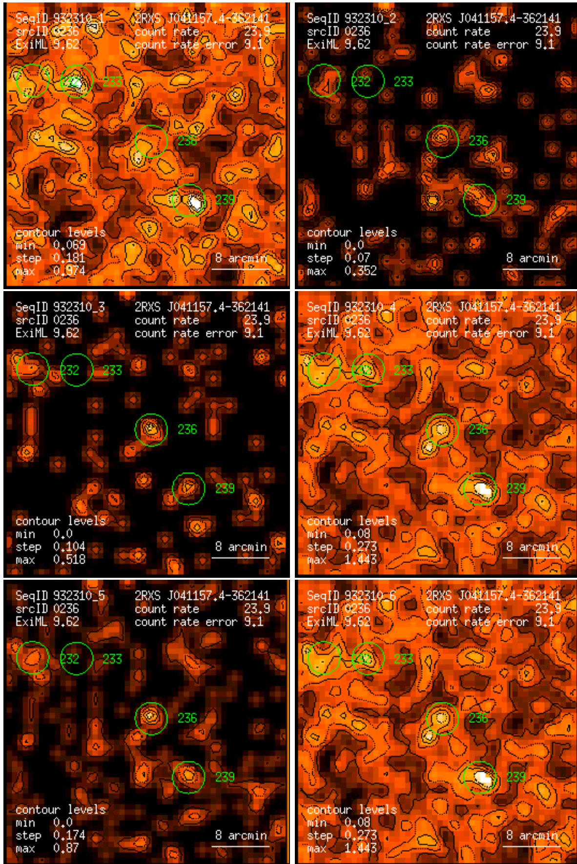
Figure 236: RASS 932310: detection 0236: band rate images, Gaussian filter: (1) PSPC channels 11 – 41, (2) 52 – 90, (3) 91 – 201, (4) 11 – 235, (5) 52 – 201, (6) 11 – 201. Broad band rates in counts/ks. Band rate contour levels in counts/ks/arcmin 2 .
