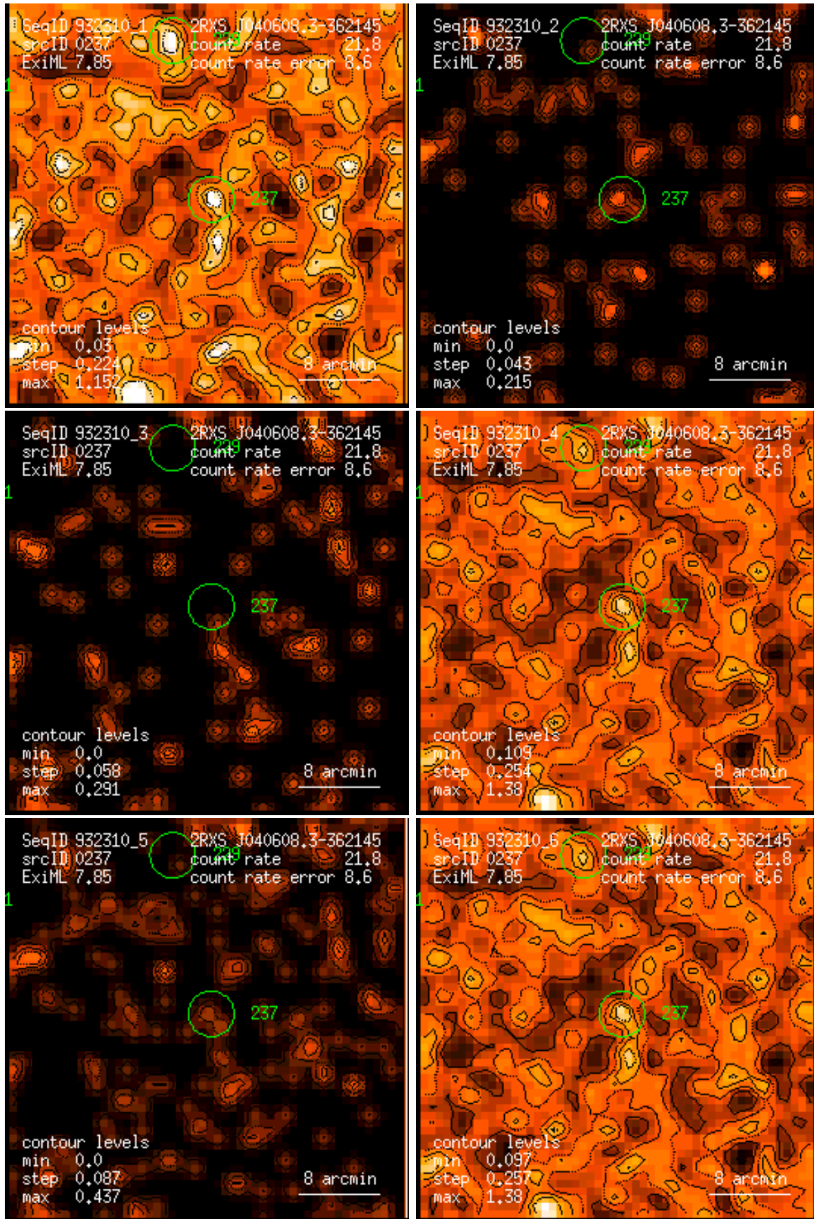
Figure 237: RASS 932310: detection 0237: band rate images, Gaussian filter: (1) PSPC channels 11 – 41, (2) 52 – 90, (3) 91 – 201, (4) 11 – 235, (5) 52 – 201, (6) 11 – 201. Broad band rates in counts/ks. Band rate contour levels in counts/ks/arcmin 2 .
